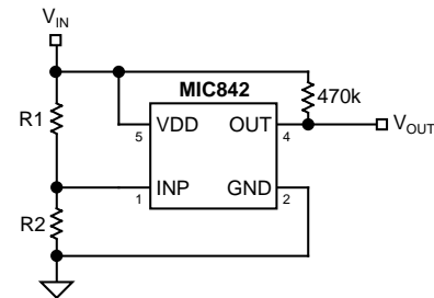
Figure 2. Example Circuit
