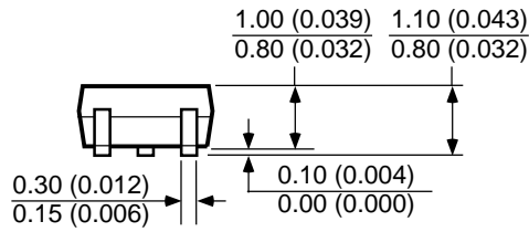
SC-70 (C5)
