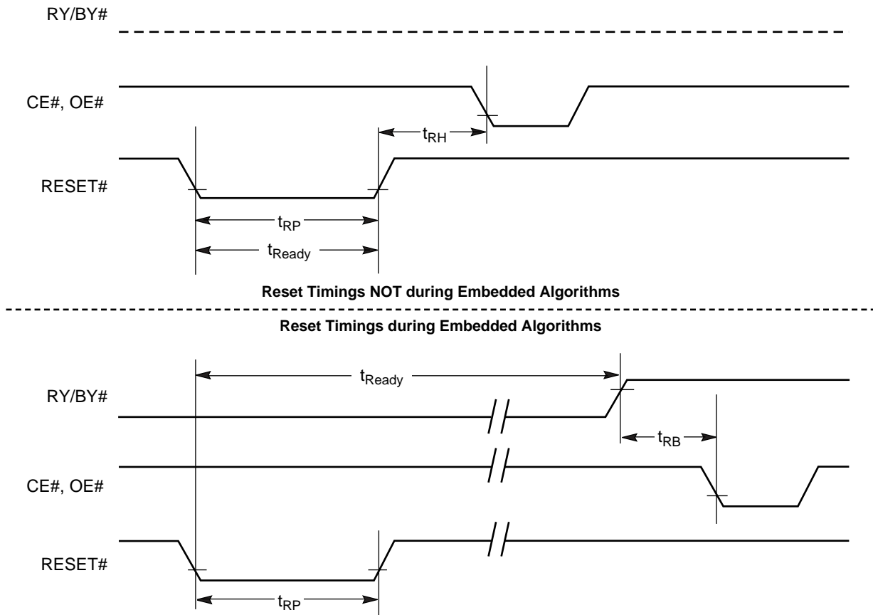
Figure 16. Reset Timings
