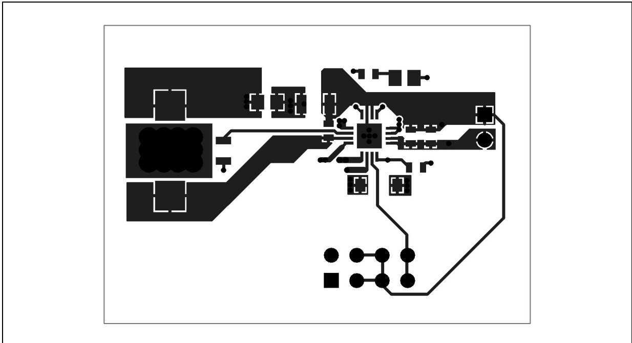
Figure 6. Top layer
