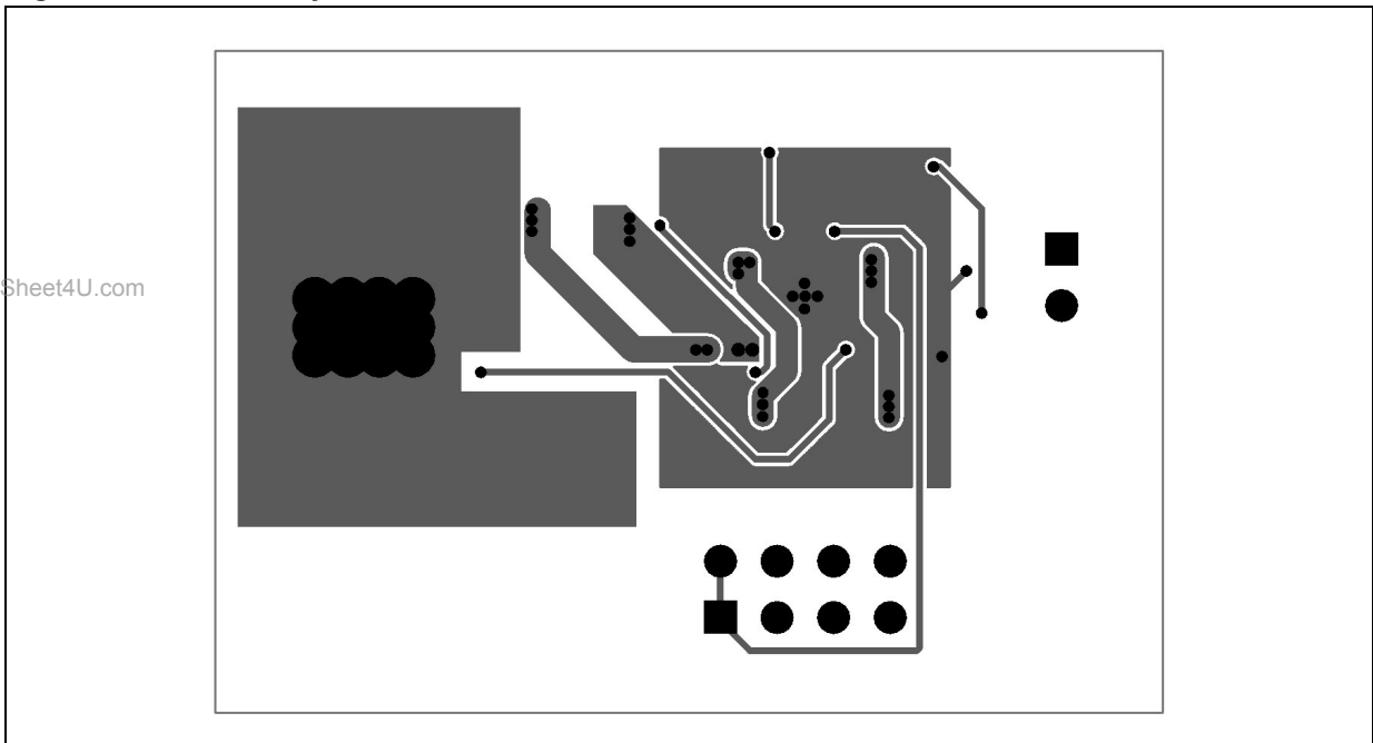
Figure 7. Bottom layer
