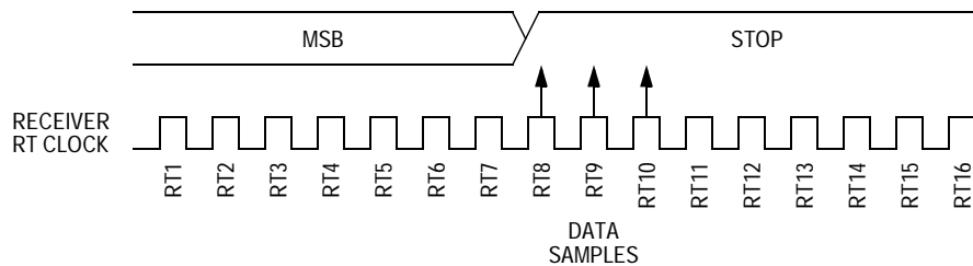
Figure 15-9. Slow Data
