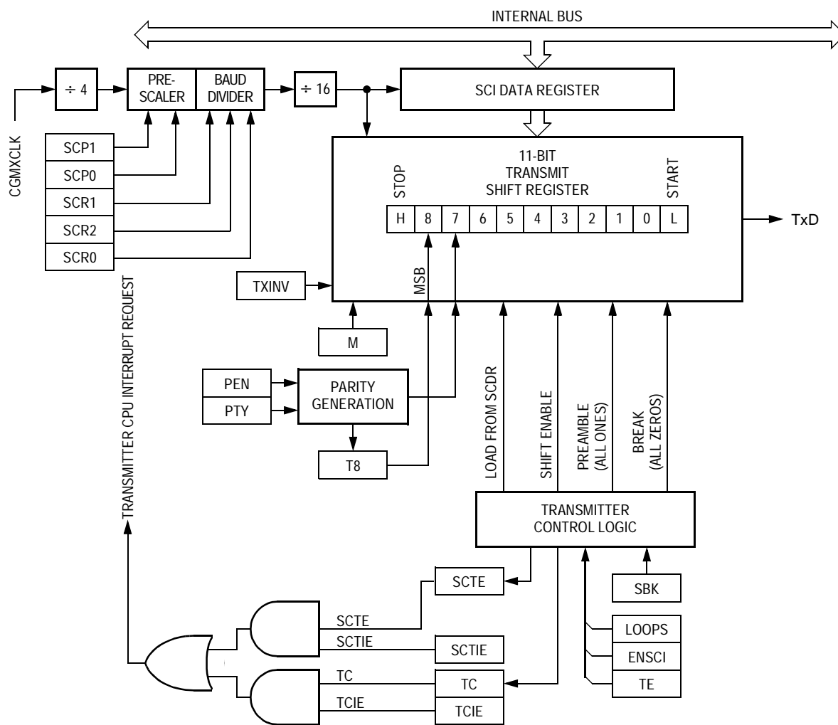
Figure 15-4. SCI Transmitter
