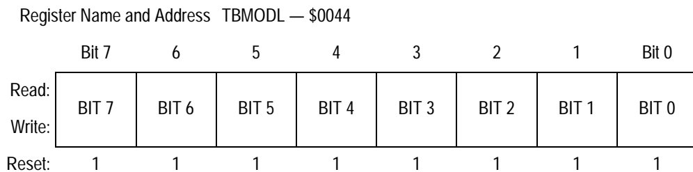
Figure 17-6. TIMB Counter Modulo Registers (TBMODH and TBMODL)
