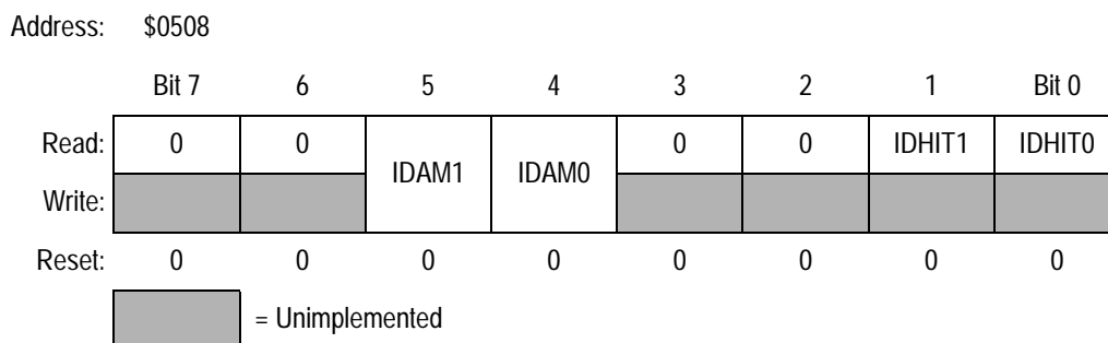
Figure 20-23. Identifier Acceptance Control Register (CIDAC)
