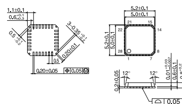
QFN28V
