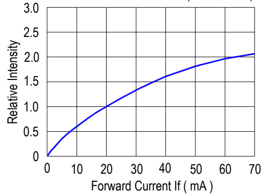
FIG. 2 Relative Intensity vs. Forward Current (Ta = 25 °C)
