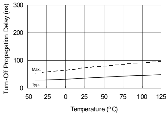
Figure 14A. Turn-Off Propagation Delay vs. Temperature
