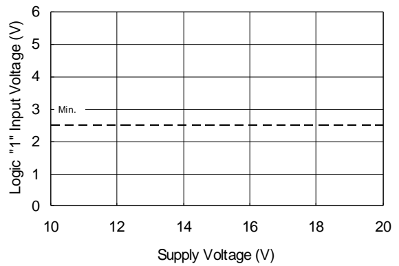
Figure 4B. Logic "1" Input Voltage vs. Supply Voltage
