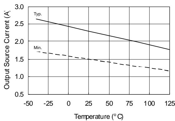
Figure 11A. Output Source Current vs. Temperature
