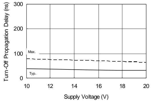
Figure 14B. Turn-Off Propagation Delay vs. Supply Voltage
