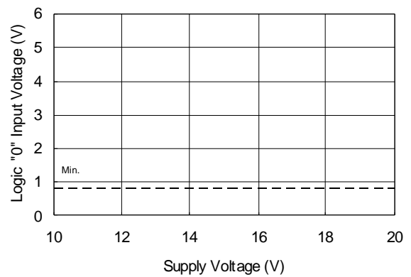
Figure 5B. Logic "0" Input Voltage vs. Supply Voltage
