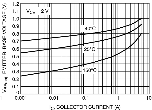
Figure 7. V_{BE(on)} Voltage
