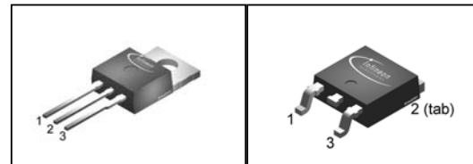
PG-TO220-3
