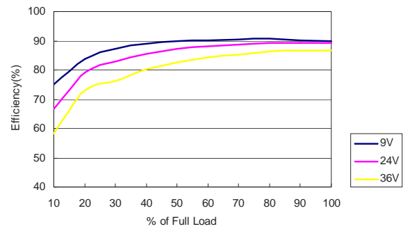
MKWI40-24S15 Efficiency vs Load Current
