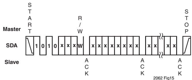
Figure 15. Write Protocol
