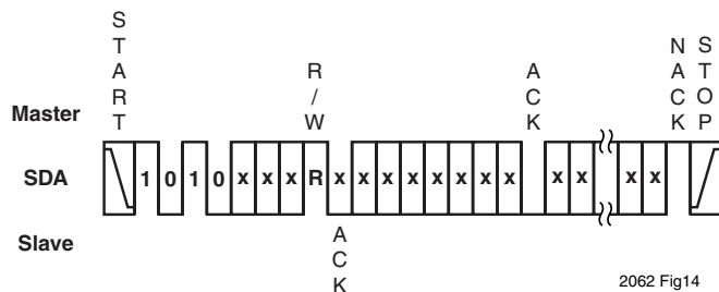
Figure 14. Read Protocol
