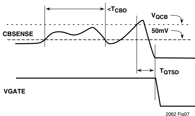
Figure 7. Circuit Breaker Quick Trip Response
