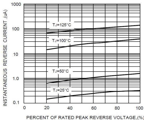
FIG.5-TYPICAL REVERSE CHARACTERISTICS
