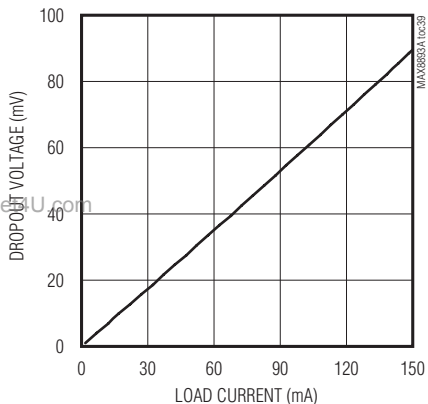
LD04 DROPOUT VOLTAGE vs. LOAD CURRENT
