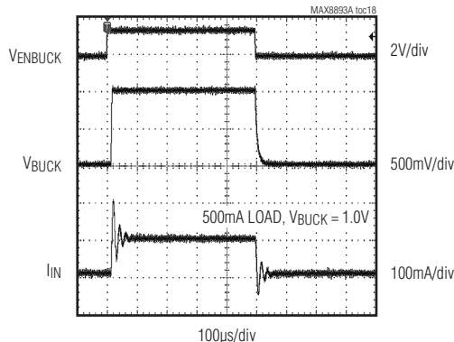
STEP-DOWN STARTUP AND SHUTDOWN WAVEFORM
