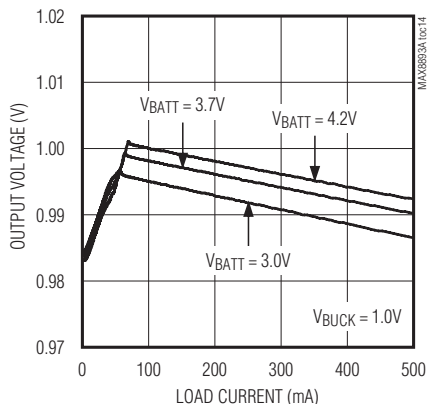
STEP-DOWN OUTPUT VOLTAGE vs. LOAD CURRENT
