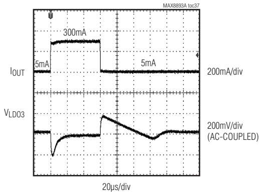
LD03 LOAD TRANSIENT WAVEFORM
