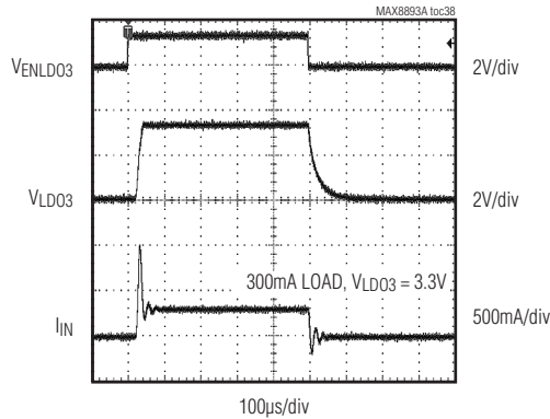
LD03 STARTUP AND SHUTDOWN WAVEFORM
