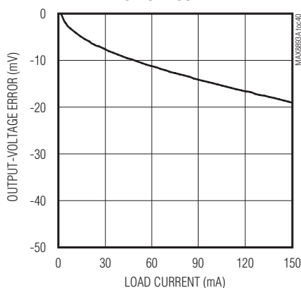
LD04 OUTPUT-VOLTAGE ERROR vs. LOAD CURRENT
