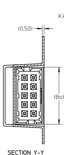
SECTION Y-Y
