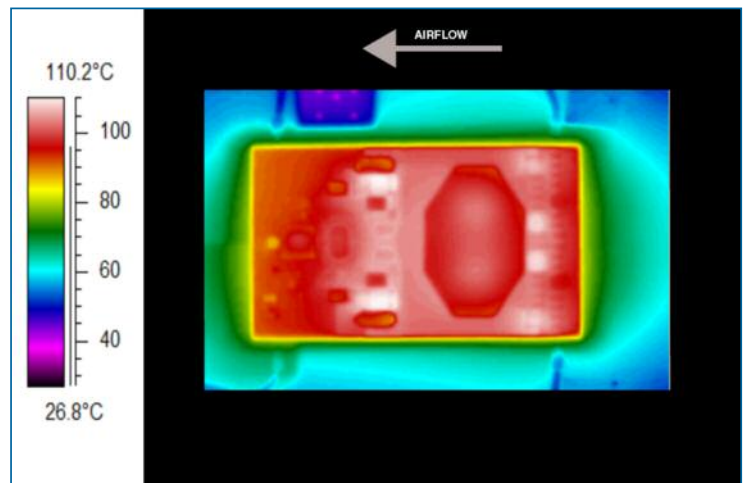
Figure 30 — Thermal plot, 600 LFM, 25 °C, 48 Vin, 760 W output power
