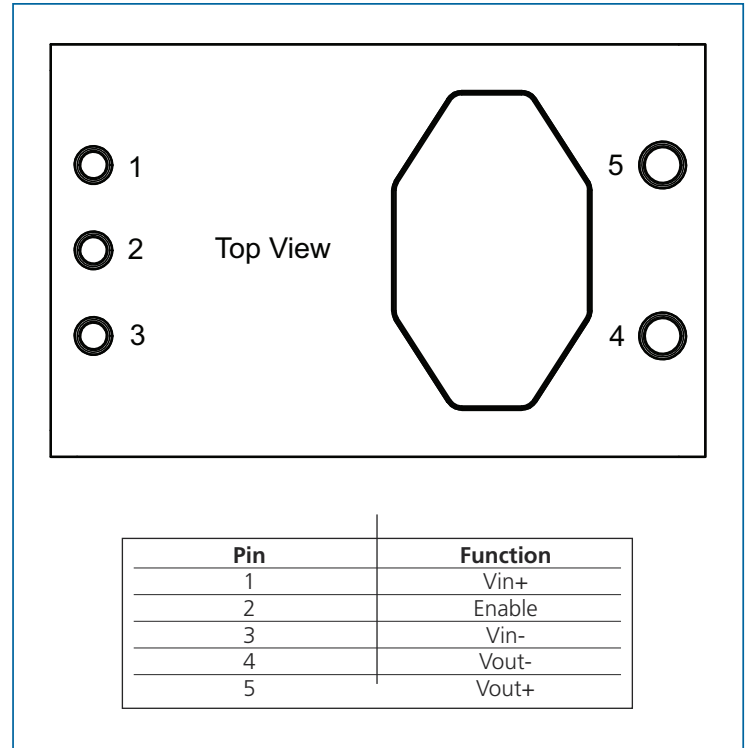
Figure 31 — IBC Pin Designations
