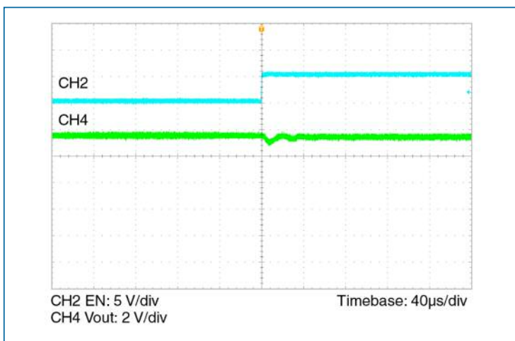
Figure 17 — Three module parallel array test. Vout change when one module is disabled. Nominal Vin, Iout = 160 A
