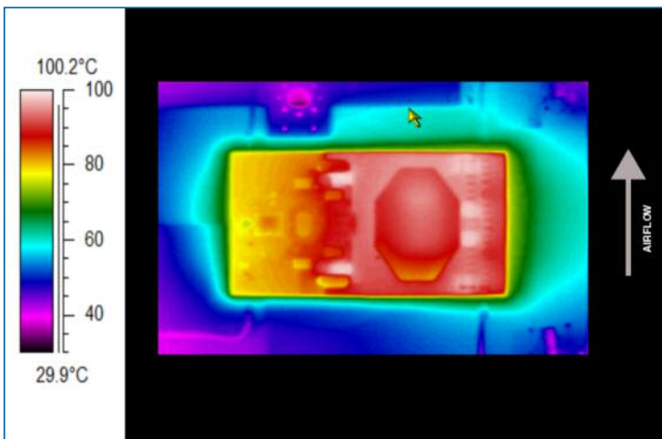
Figure 29 — Thermal plot, 600 LFM, 25 °C, 48 Vin, 760 W output power
