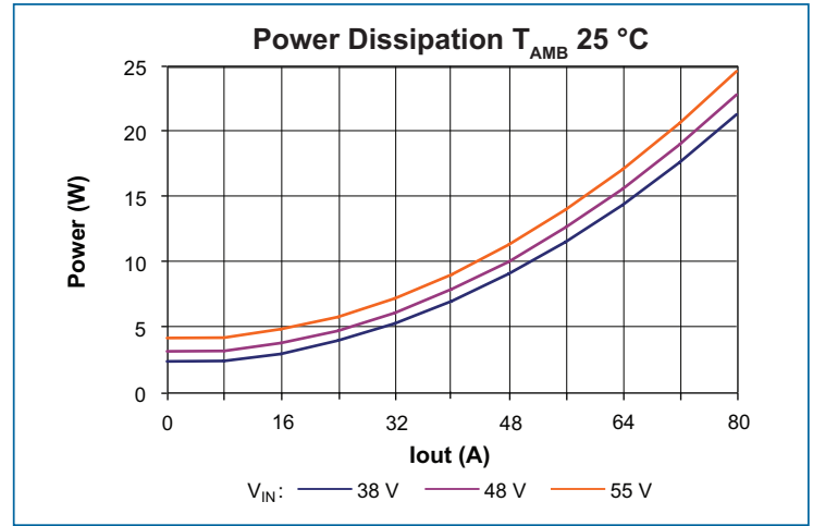
Figure 2 — Power Dissipation vs. output current
