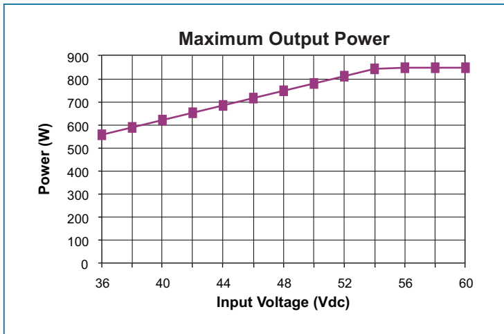
Figure 3 — Maximum output power vs. input voltage
