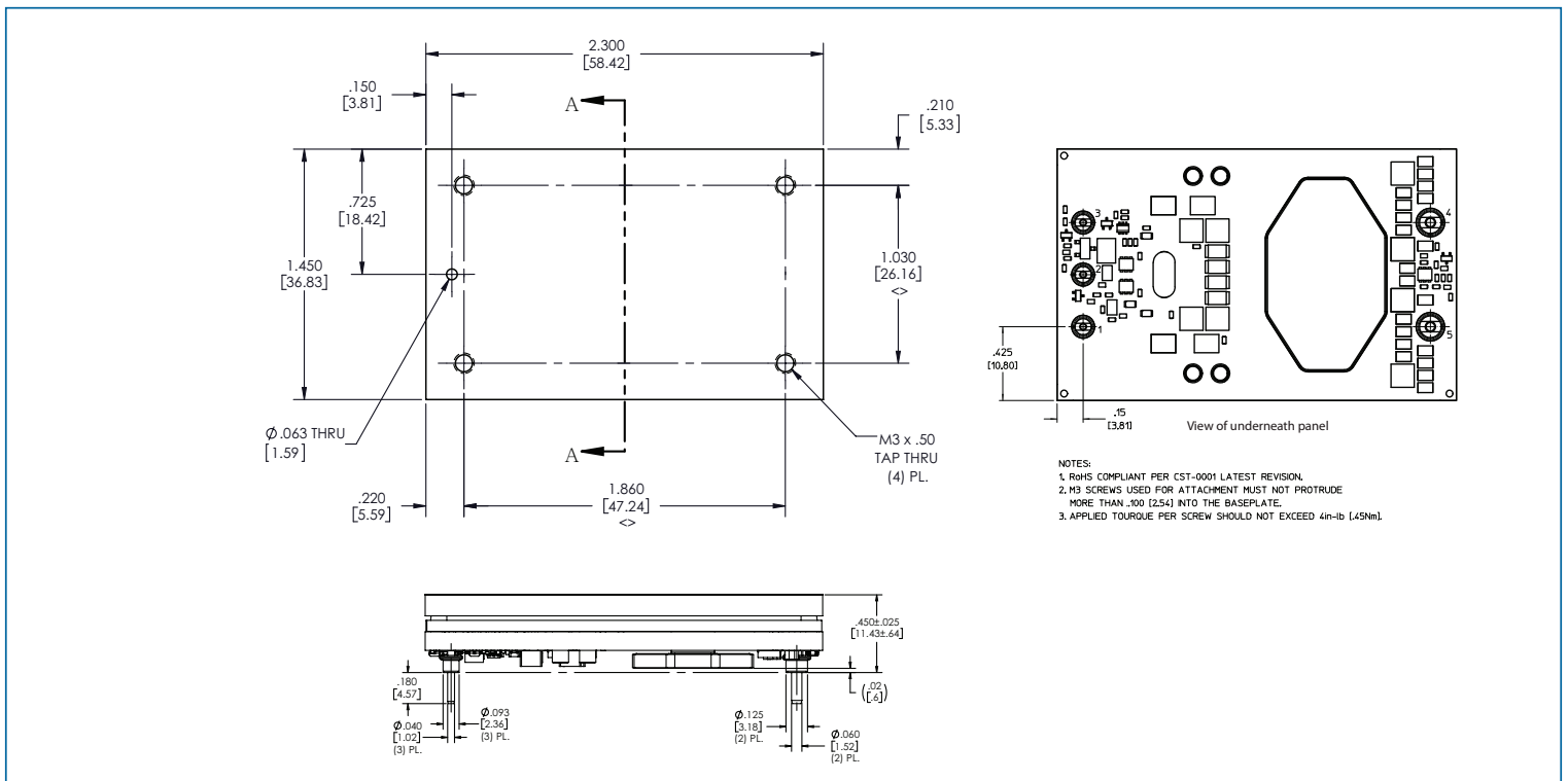
Figure 33 — IBC outline drawing - baseplate option
