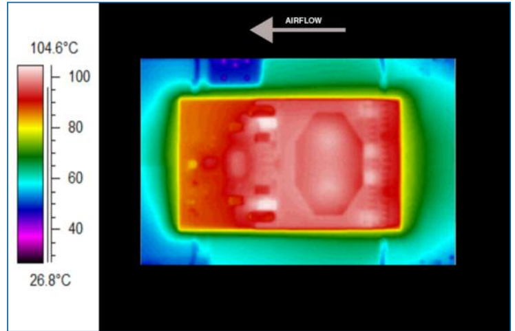
Figure 28 — Thermal plot, 400 LFM, 25 °C, 48 Vin, 670 W output power
