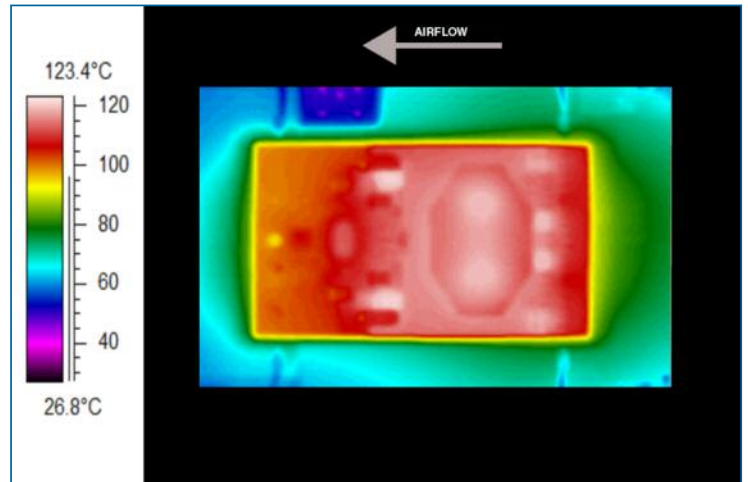
Figure 26 — Thermal plot, 200 LFM, 25 °C, 48 Vin, 670 W output power
