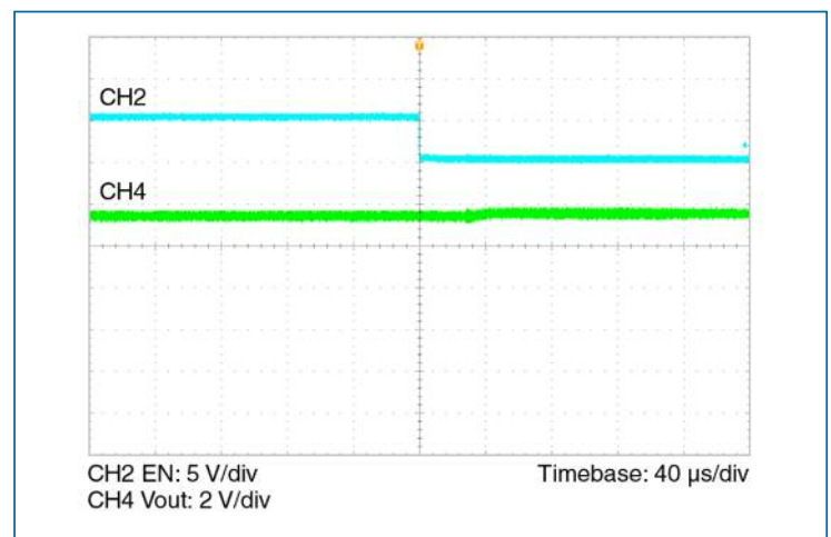
Figure 18 — Three module parallel array test. Vout change with two modules operating and a third module enabled. Nominal Vin, Iout = 160 A
