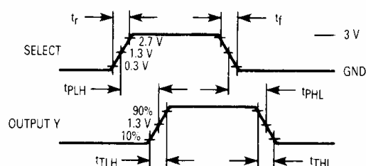
Figure 2. Switching Waveforms
