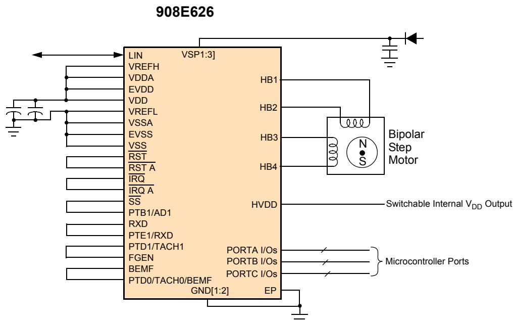
Figure 1. 908E626 Simplified Application Diagram
