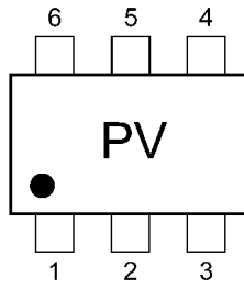
Fig. 6.1 Marking
