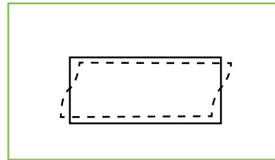
Thickness Shear Mode
