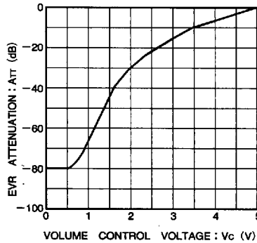
Fig. 5 EVR attenuation characteristic
