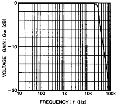
Fig. 4 Voltage gain vs. frequency characteristics
