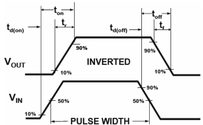
Switch Waveforms:
