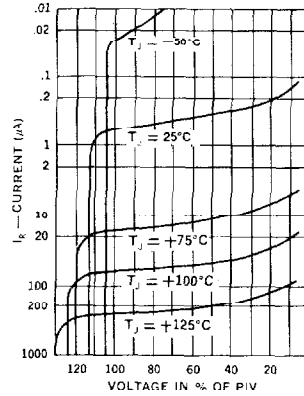
Typical Reverse Current vs Voltage
