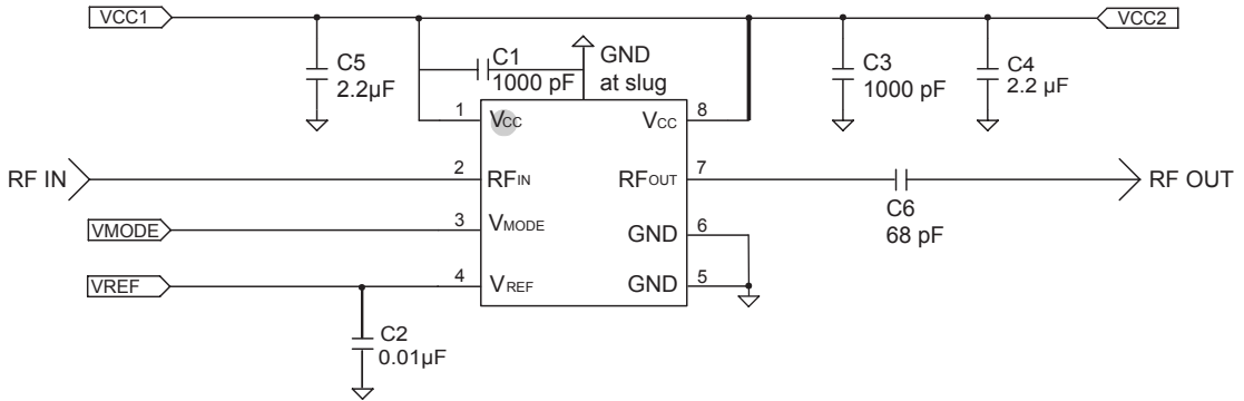
Figure 3: Application Circuit
