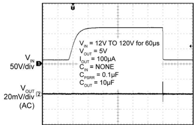
Time (10µs/div)
