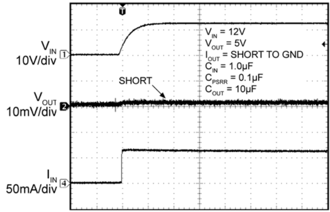
Time (40ms/div)
