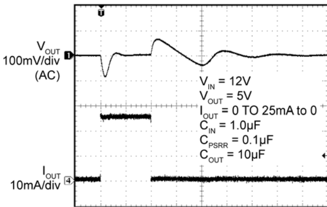
Time (100µs/div)
