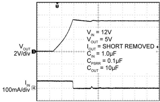
Time (400µs/div)
