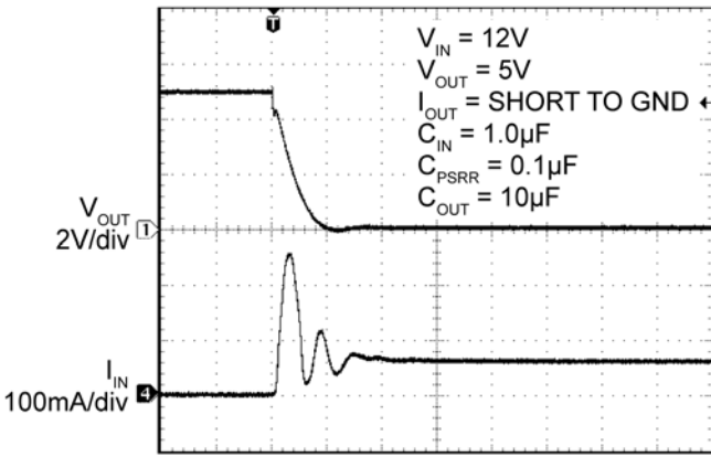
Time (4.0µs/div)
