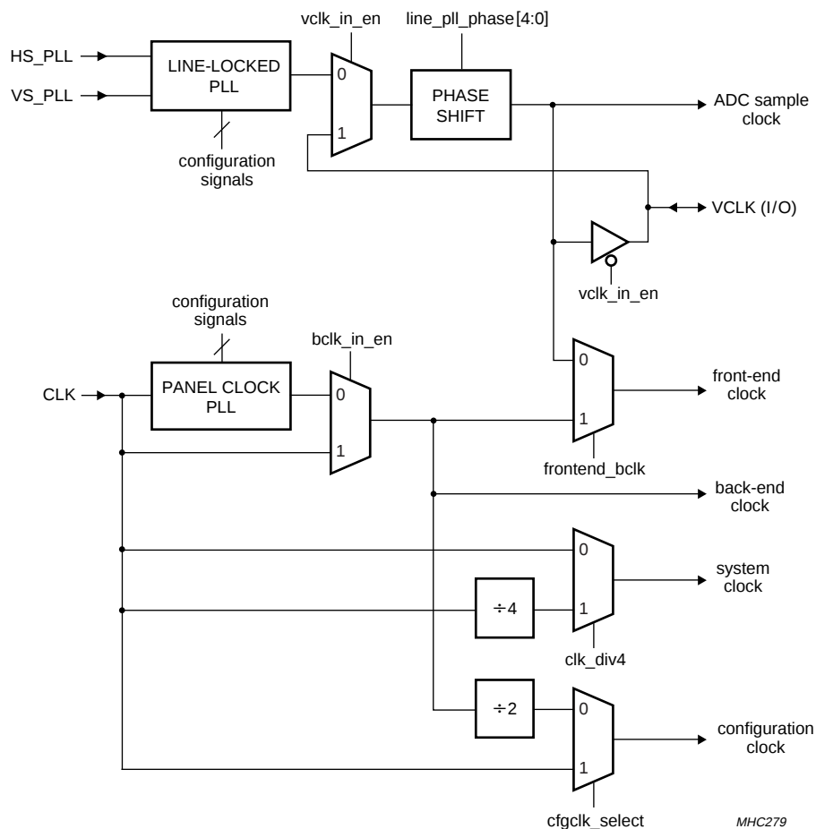
Fig.5 Clock distribution.
