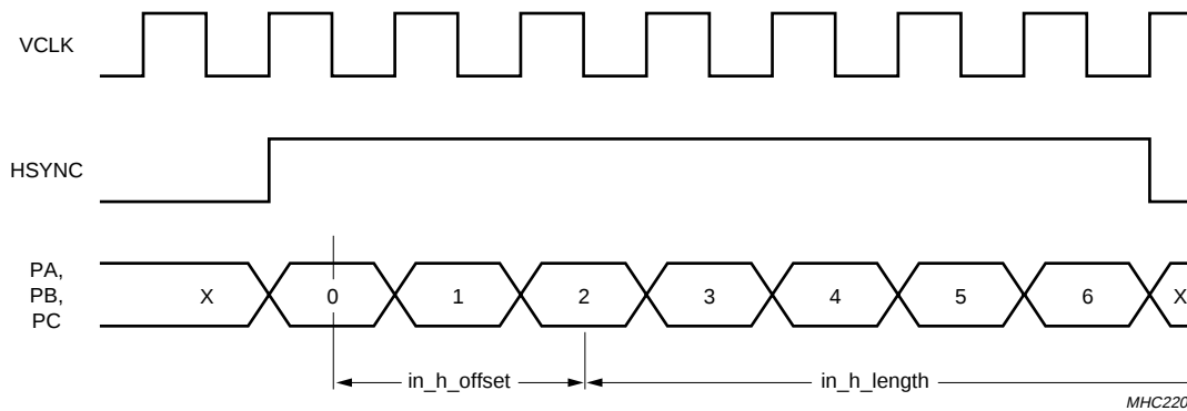
Fig.13 RGB input port timing using a data enable signal (connected to HSYNC).
