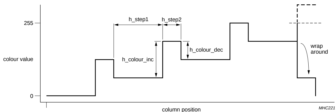
Fig.14 Picture generator ramp and ripple pattern (horizontal generator).
