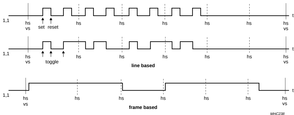
Fig.31 Examples for CSG0/1 outputs.
