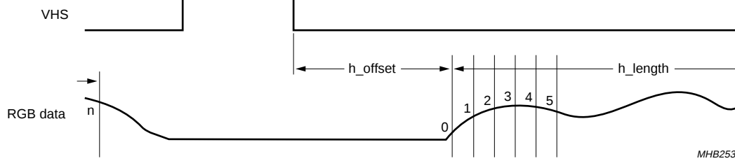
Fig.12 RGB data sampling (hsync_edge = 0).
