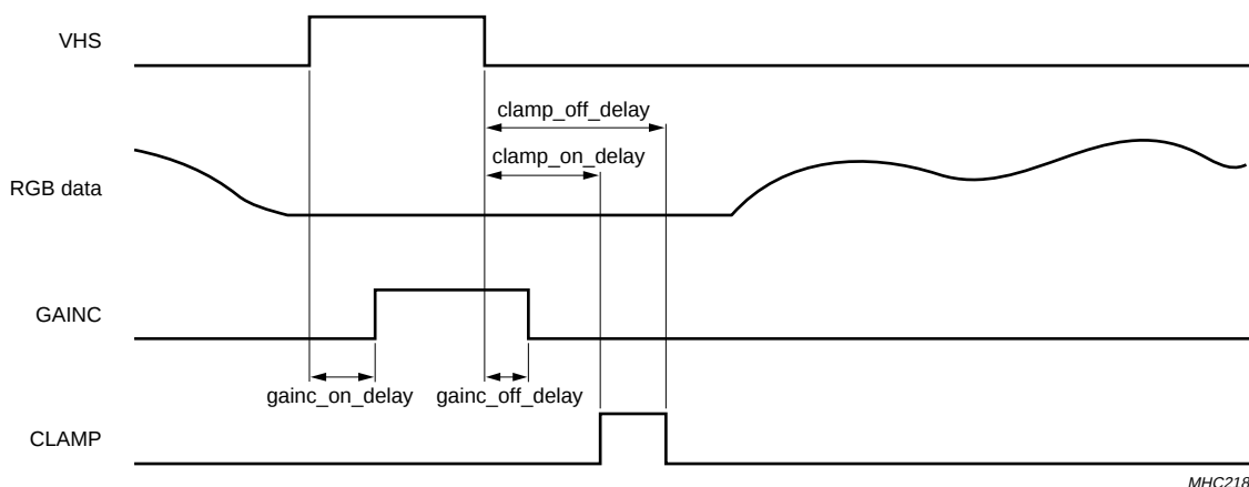
Fig.10 Gain adjustment and clamp pulse generation.
