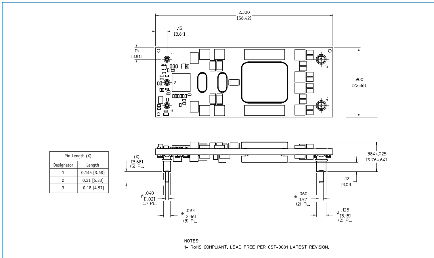
Figure 32 — IBC outline drawing
