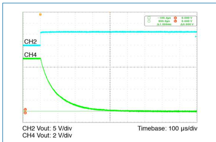
Figure 10 — Undershoot at turn off at nominal line, 15% load
