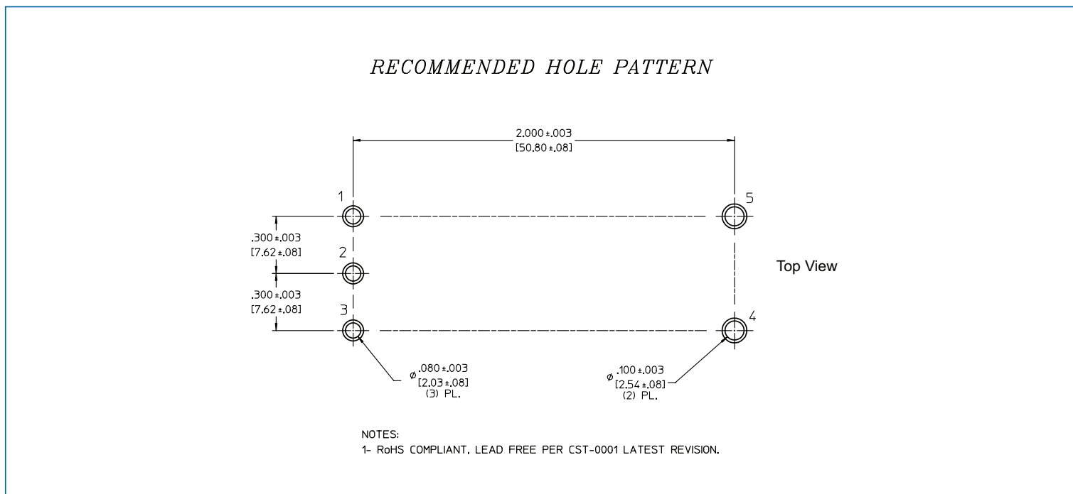
Figure 33 — IBC PCB recommended hole pattern
