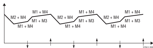
Figure 5. Buck-Boost Operation ( V_{IN} \geq V_{OUT} )
