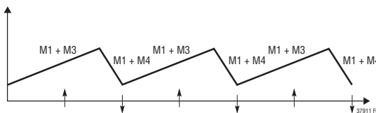
Figure 6. Boost Operation ( V_{IN} < V_{OUT} )
