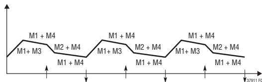
Figure 4. Buck-Boost Operation ( V_{IN} \leq V_{OUT} )
