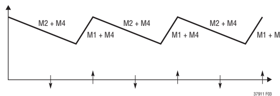
Figure 3. Buck Operation ( V_{IN} > V_{OUT} )
