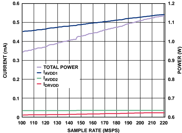
Figure 62. Supply Current vs. f_{SAMPLE} for f_{IN} = 5 MHz, AD9467-200
