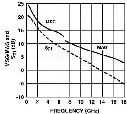
Figure 23. MSG/MAG and |S_{21}|^2 vs. Frequency at 3 V, 20 mA.
