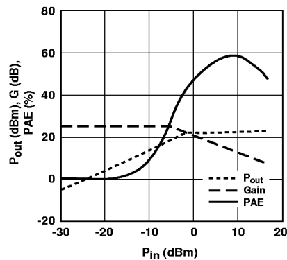
Figure 21. Swept Power Tuned for Power at 2 GHz, V_{DS} = 4 V, I_{DSQ} = 60 mA.
