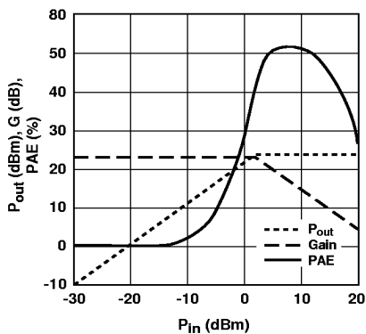
Figure 20. Swept Power Tuned for Power at 2 GHz, V_{DS} = 4 V, I_{DSQ} = 120 mA.
