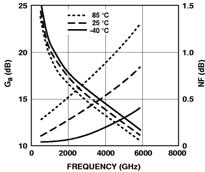
Figure 14. F_{min} and G_a vs. Frequency and Temperature at V_{DS} = 4 V, I_{DS} = 60 mA.
