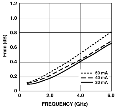
Figure 12. F_{min} vs. Frequency and Current at 4 V.
