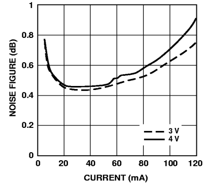
Figure 8. Noise Figure vs. Current ( I_d ) and Voltage ( V_{DS} ) at 2 GHz. [1,2]
