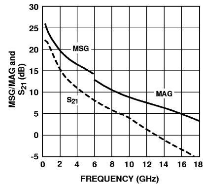
Figure 25. MSG/MAG and |S_{21}|^2 vs. Frequency at 4 V, 40 mA.
