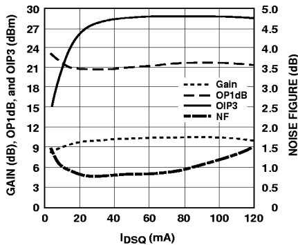
Figure 17. NF, Gain, OP1dB and OIP3 vs. I_{DSQ} at 4 V and 5.8 GHz Tuned for Noise Figure. [1]
