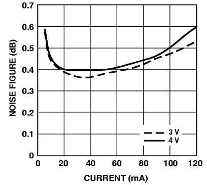
Figure 11. Noise Figure vs. Current ( I_d ) and Voltage ( V_{DS} ) at 900 MHz. [1,2]
