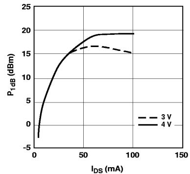
Figure 19. P_{1dB} vs. I_{DS} Active Bias Tuned for min NF @ 4 V, 60 mA at 900 MHz.
