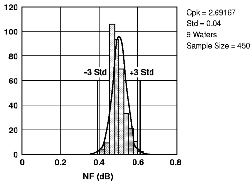
Figure 3. NF @ 2 GHz, 4 V, 60 mA. LSL=0.1, Nominal=0.47, USL=0.8
