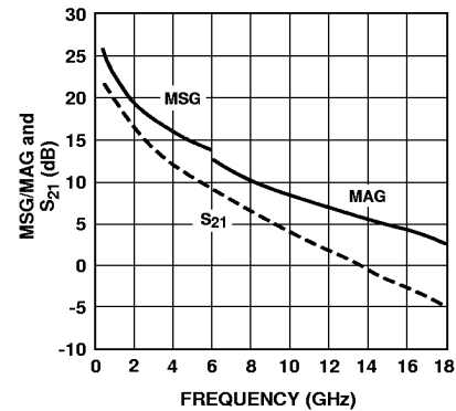
Figure 24. MSG/MAG and |S_{21}|^2 vs. Frequency at 3 V, 40 mA.
