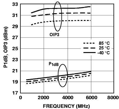
Figure 15. P_{1dB} , IP_3 vs. Frequency and Temperature at V_{DS} = 4 V, I_{DS} = 60 mA. [1]
