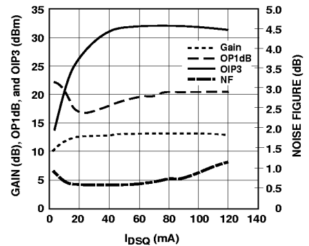
Figure 16. NF, Gain, OP1dB and OIP3 vs. I_{DSQ} at 4 V and 3.9 GHz Tuned for Noise Figure. [1]
