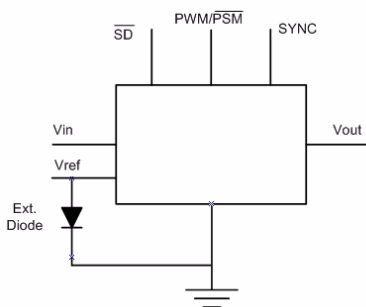
Pin Configuration for V_o = 0.8V
