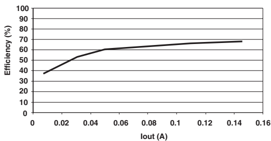
Efficiency Vs. Iout* Vin = 4.0V; Vout = 1.2V
