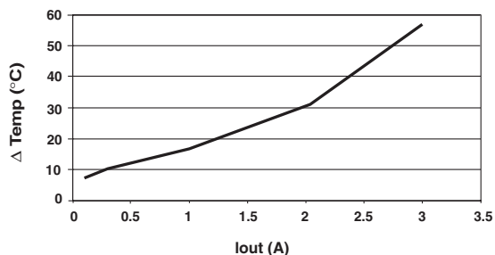
Δ Temp Vs. Iout*
