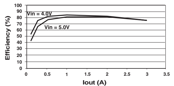
Efficiency Vs. Iout* Vin = 4.0V; Vout = 1.2V
