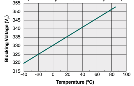
Typical Blocking Voltage vs. Temperature (Form-A: I_F=0mA , Form-B: I_F=5mA )
