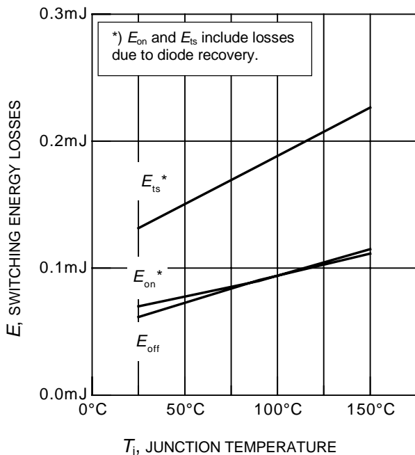
Figure 15. Typical switching energy losses as a function of junction temperature (inductive load, V_{CE} = 400\text{V} , V_{GE} = 0/+15\text{V} , I_C = 4\text{A} , R_G = 67\Omega )
