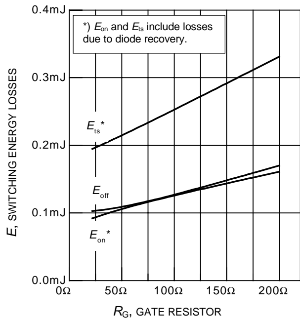
Figure 14. Typical switching energy losses as a function of gate resistor (inductive load, T_j = 150^\circ\text{C} , V_{CE} = 400\text{V} , V_{GE} = 0/+15\text{V} , I_C = 4\text{A} )
