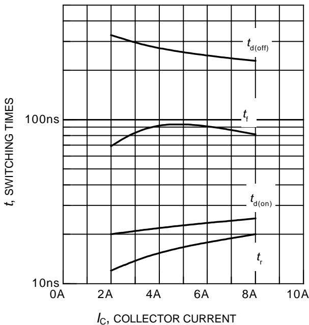
Figure 9. Typical switching times as a function of collector current (inductive load, T_j = 150^\circ\text{C} , V_{CE} = 400\text{V} , V_{GE} = 0/+15\text{V} , R_G = 67\Omega )
