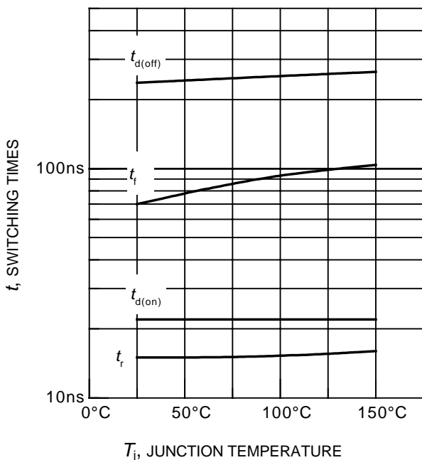
Figure 11. Typical switching times as a function of junction temperature (inductive load, V_{CE} = 400\text{V} , V_{GE} = 0/+15\text{V} , I_C = 4\text{A} , R_G = 67\Omega )
