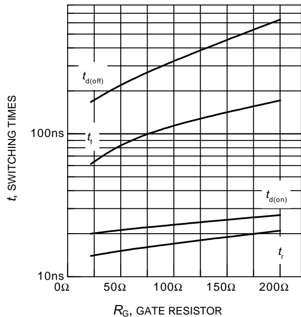
Figure 10. Typical switching times as a function of gate resistor (inductive load, T_j = 150^\circ\text{C} , V_{CE} = 400\text{V} , V_{GE} = 0/+15\text{V} , I_C = 4\text{A} )
