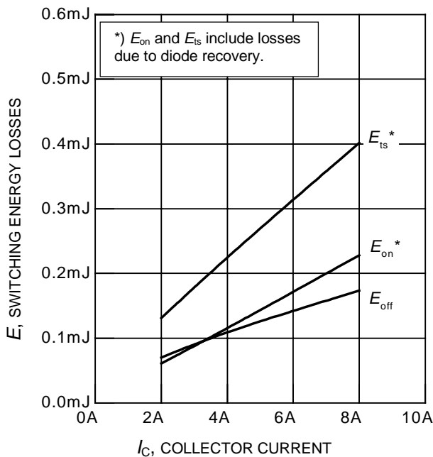
Figure 13. Typical switching energy losses as a function of collector current (inductive load, T_j = 150^\circ\text{C} , V_{CE} = 400\text{V} , V_{GE} = 0/+15\text{V} , R_G = 67\Omega )
