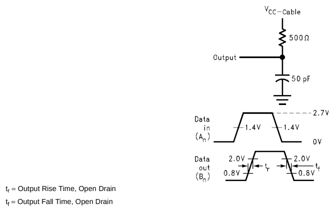
FIGURE 8. Ports A to B and A to Y Rise and Fall Test Load and Waveforms for Open Drain Outputs
