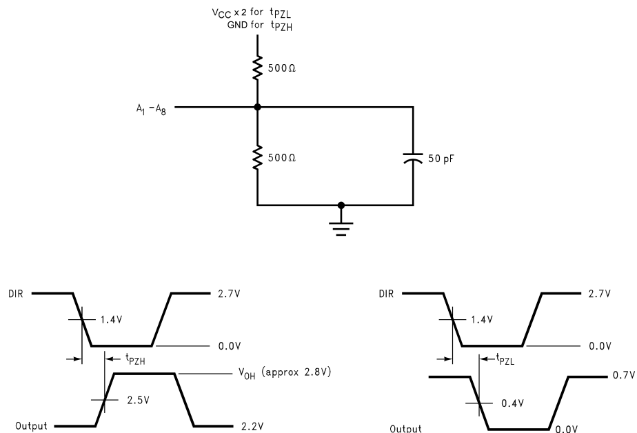
FIGURE 10. t PZH and t PLZ Test Load and Waveforms, DIR to A 1 -A 8
