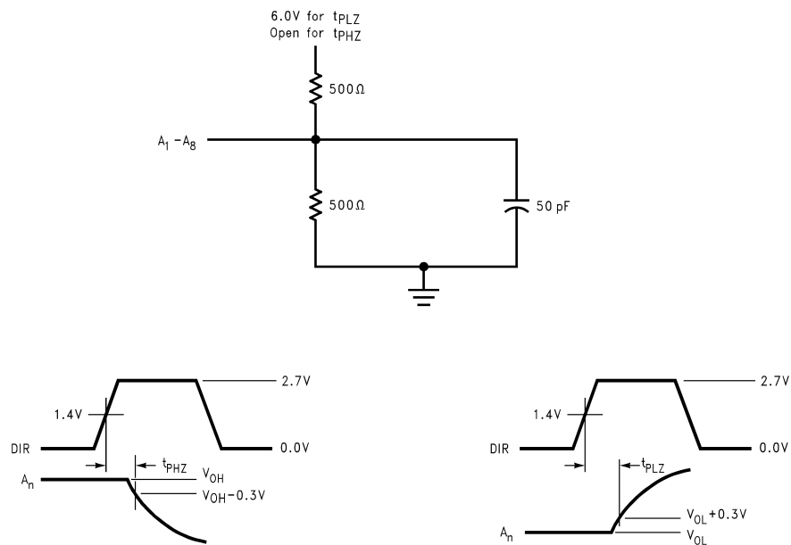
FIGURE 9. t_{PHZ} and t_{PLZ} Test Load and Waveforms, DIR to A_1-A_8
