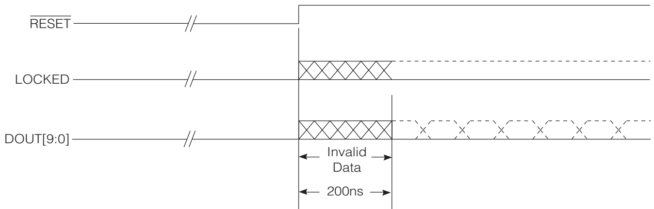
Figure 3-20: Reset Timing
