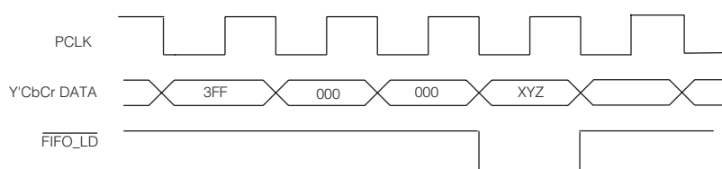
Figure 3-4: \overline{\text{FIFO\_LD}} Pulse Timing
