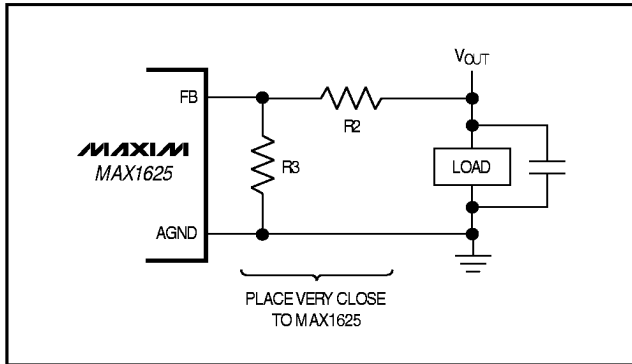
Figure 7. MAX1625 Adjustable Output Operation
