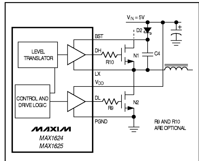
Figure 5. Boost Supply for Gate Drivers
