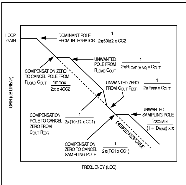
Figure 8. MAX1624/MAX1625 Bode Plot with Compensation Poles and Zeros
