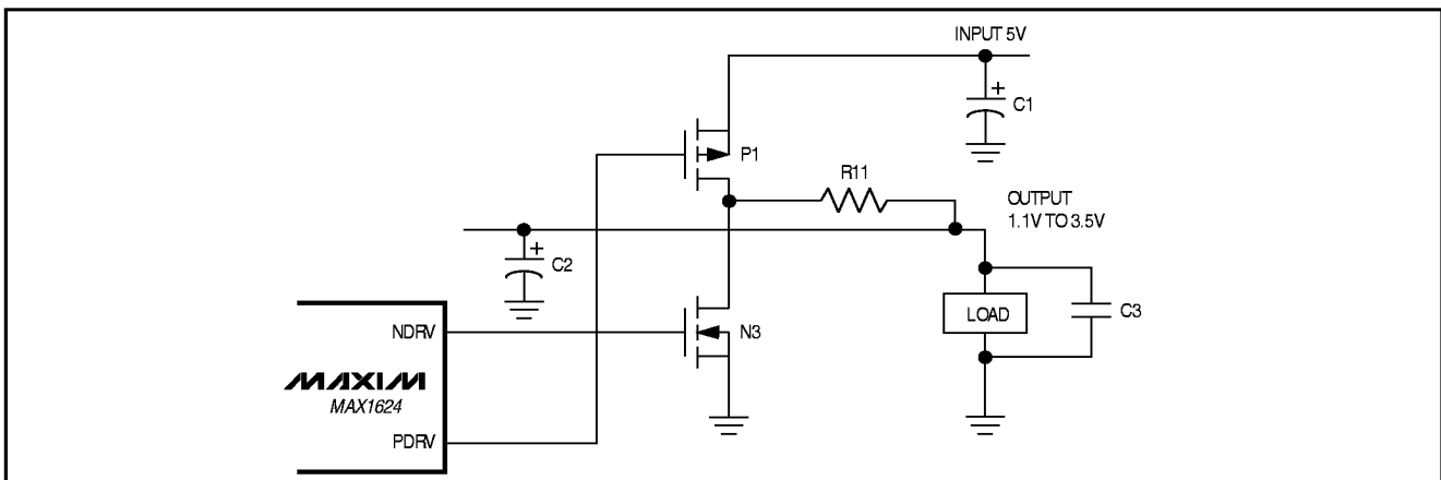
Figure 10. GlitchCatcher Circuit
