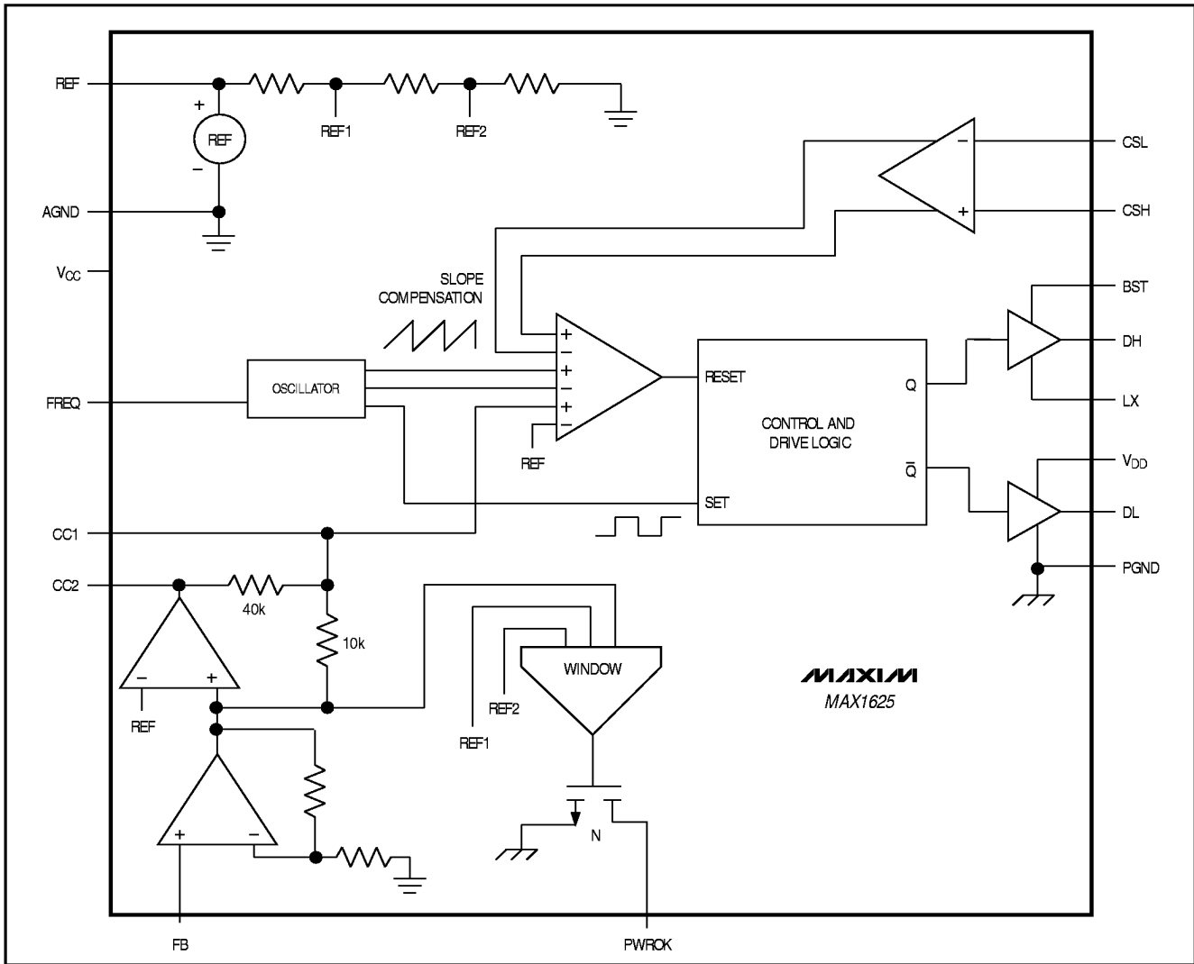
Figure 4. MAX1625 Simplified Block Diagram
