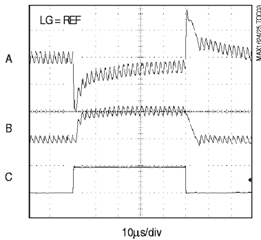
MAX1624 LOAD-TRANSIENT RESPONSE (WITHOUT GLITCHCATCHER) (1.1V)
