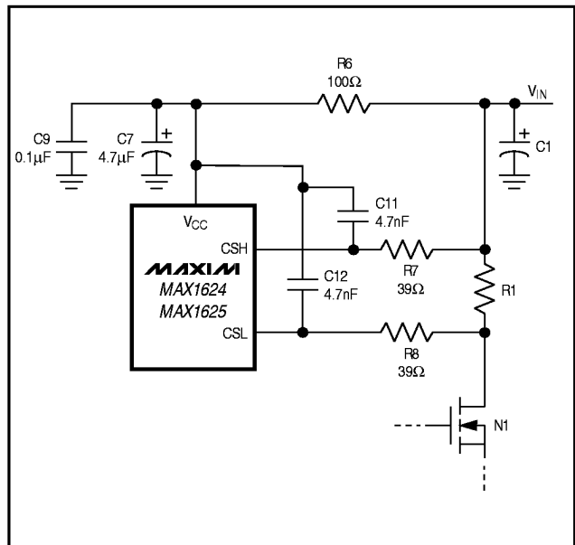
Figure 6. Current-Sense Filter
