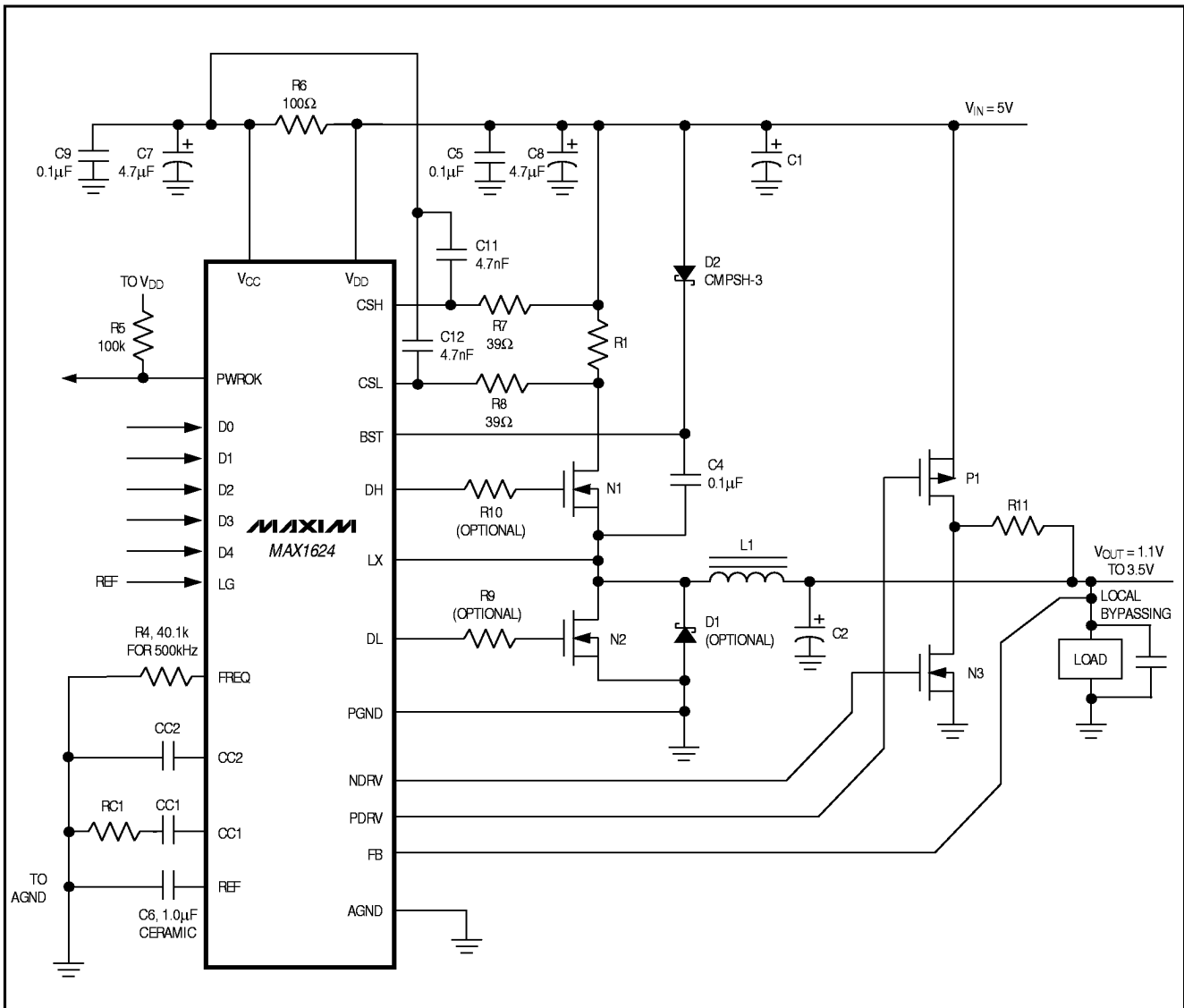
Figure 1. MAX1624 Standard Application Circuit
