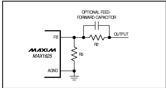
Figure 9. MAX1625 Optional Feed-Forward Compensation Capacitors
