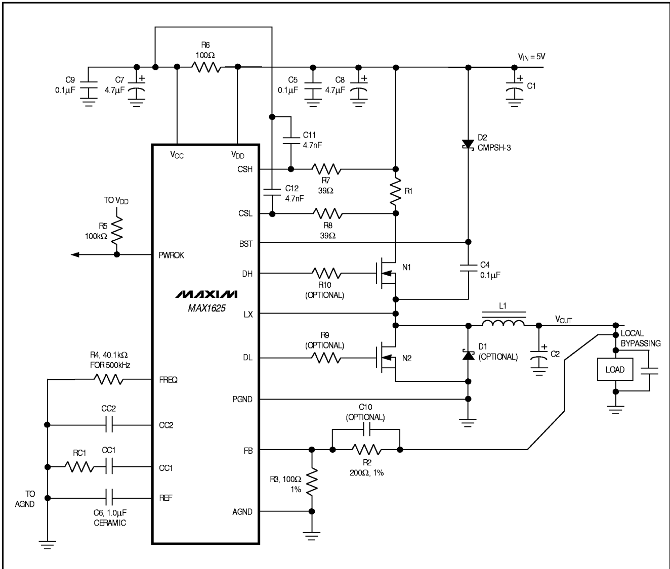
Figure 2. MAX1625 Standard Application Circuit
