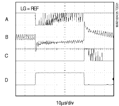
MAX1624 LOAD-TRANSIENT RESPONSE DETAIL (WITH GLITCHCATCHER) (1.1V)
