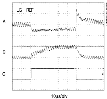
MAX1624 LOAD-TRANSIENT RESPONSE (WITH GLITCHCATCHER) (1.1V)
