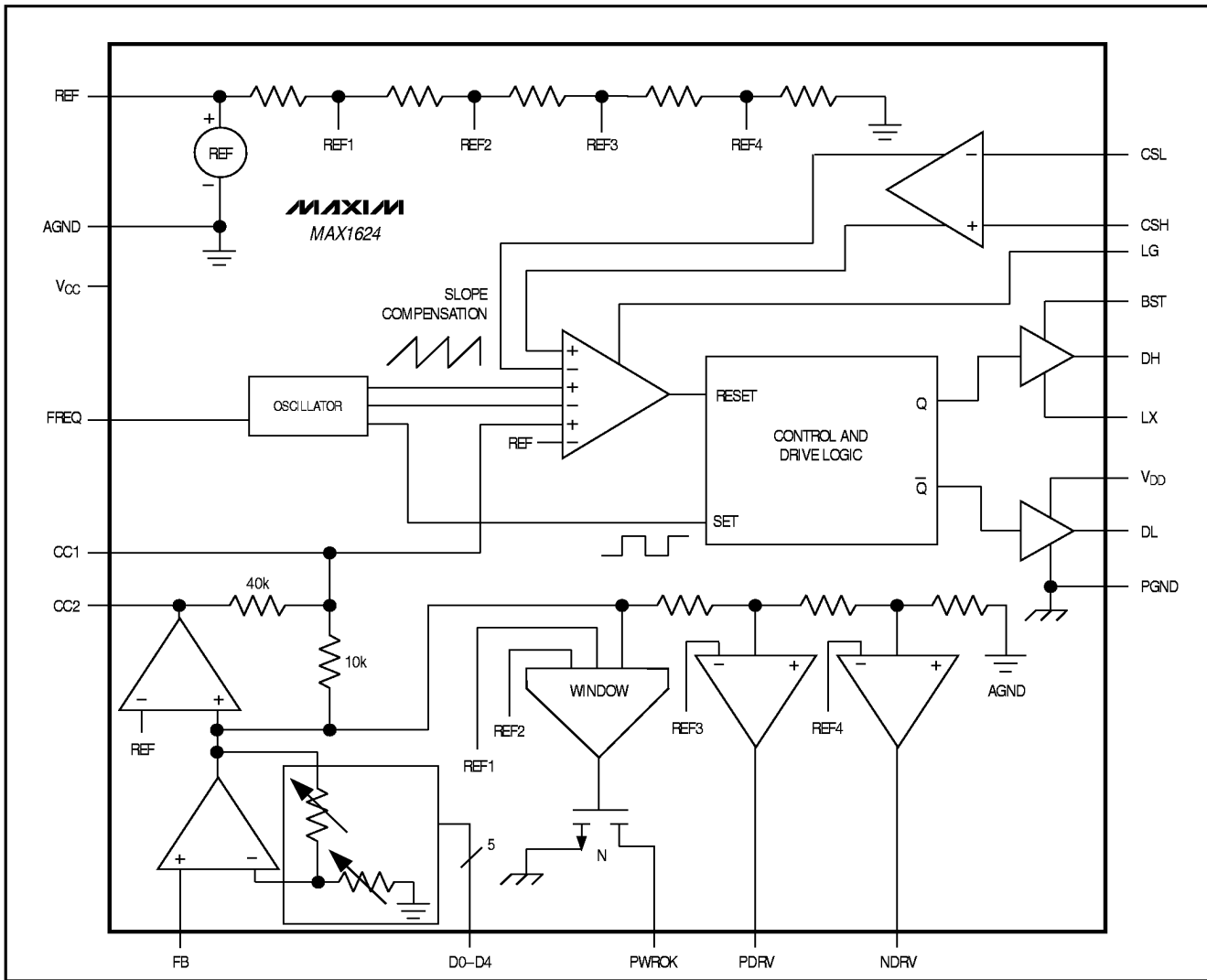
Figure 3. MAX1624 Simplified Block Diagram
