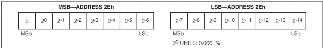
Figure 55. CGAIN Register Format (Input)
