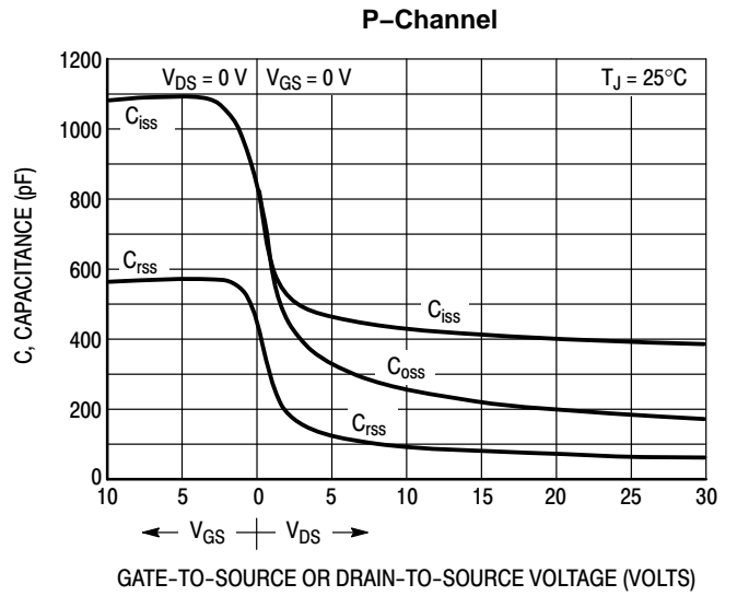
Figure 7. Capacitance Variation
