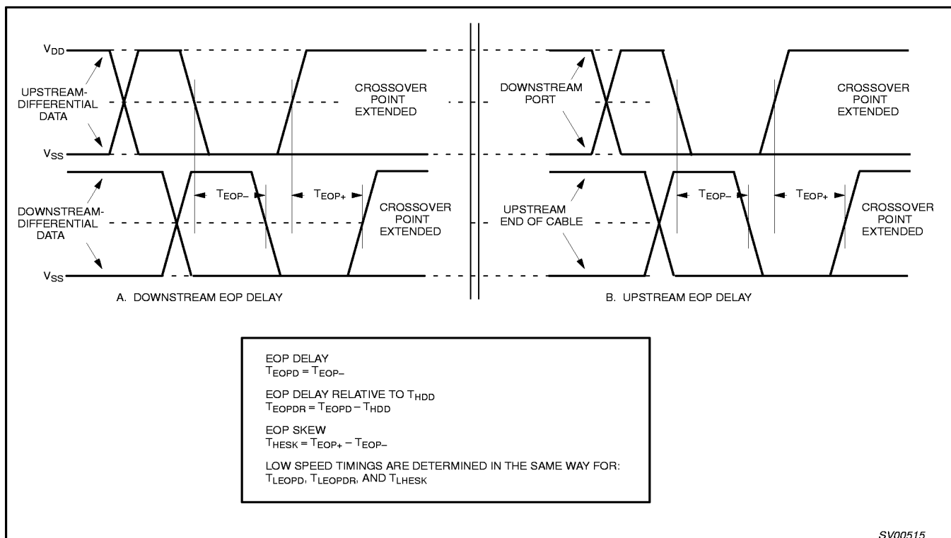
Figure 3. Hub EOP Delay and EOP Skew
