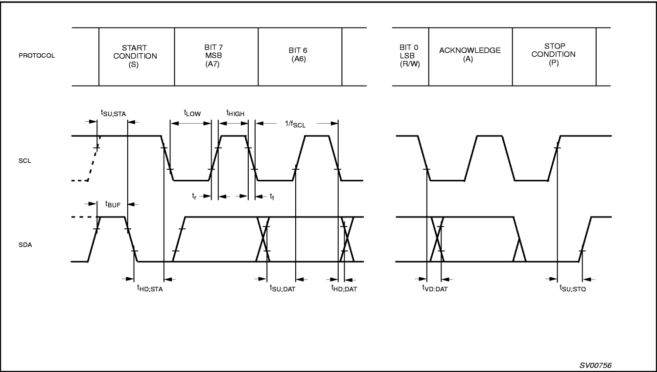
Figure 4. I 2 C-bus timing diagram
