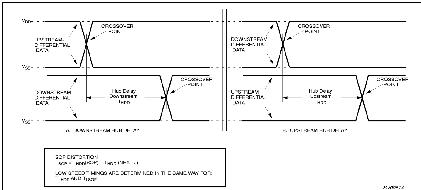
Figure 2. Hub Differential Data Delay and SOP distortion
