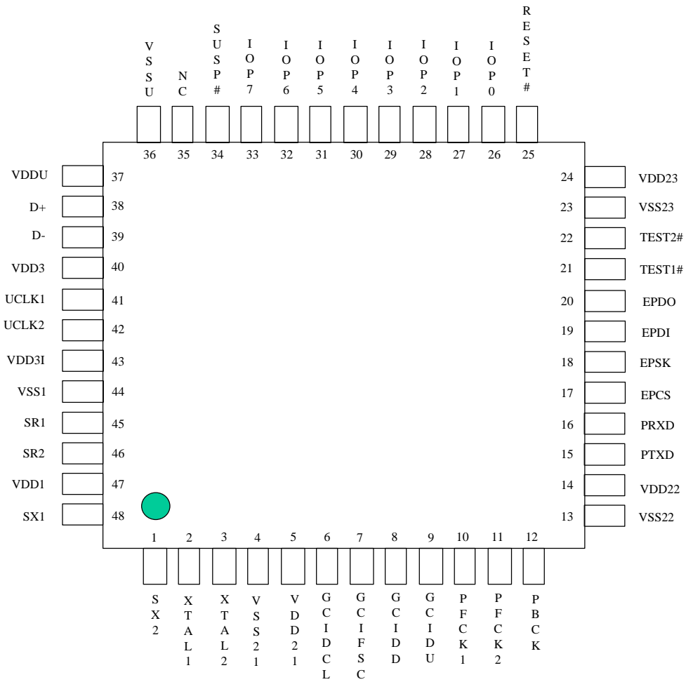
FIG.3.1 W6694 PIN OUT
