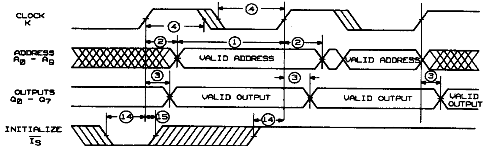
Timing Set 4. Using Synchronous Initialize Am27S37 Only
