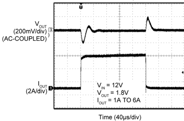
Transient Response
