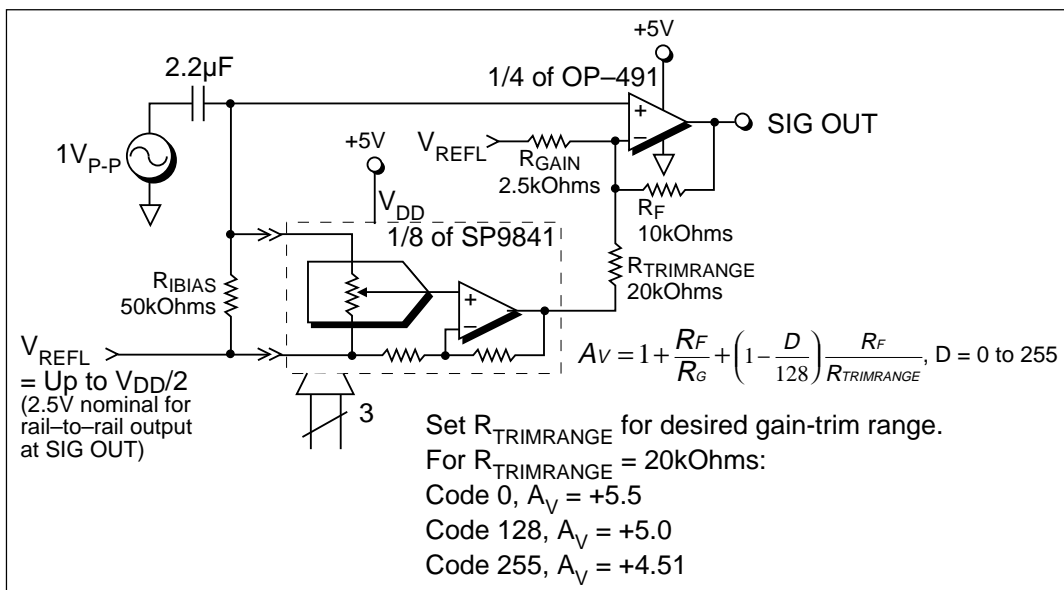
Figure 10. Adjustable Gain of External Non-Inverting Opamp Circuit; V_{OUT} = Rail-to-rail.
