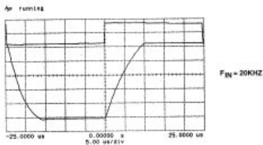
Plot 23. Pulse Response — a) C_{LOAD} = 47,000pF ; b) C_{LOAD} = 47,000pF , R_{LOAD} = 1kOhm ; c) 15 Ohms in series with C_{LOAD} = 47,000pF ; d) R_{LOAD} = 1kOhm , 15 Ohms in series with C_{LOAD} = 47,000pF .
