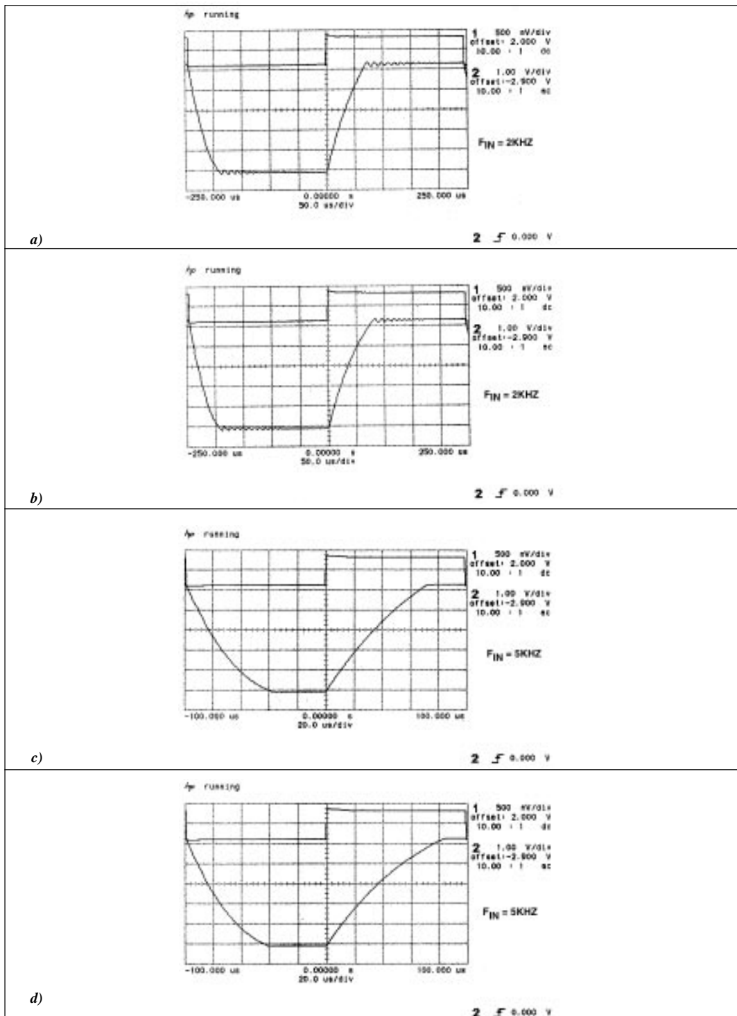
Plot 24. Pulse Response — a) C_{LOAD} = 0.47\mu F ; b) C_{LOAD} = 0.47\mu F , R_{LOAD} = 1k\Omega ; c) 8.2 Ohms in series with C_{LOAD} = 0.47\mu F ; d) R_{LOAD} = 1k\Omega , 8.2 Ohms in series with C_{LOAD} = 0.47\mu F .
