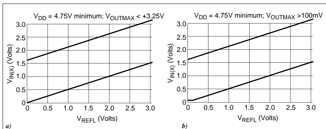
Figure 3. Reference Voltages a) Normal Operation; b) Maximum Linearity Near Code 1
