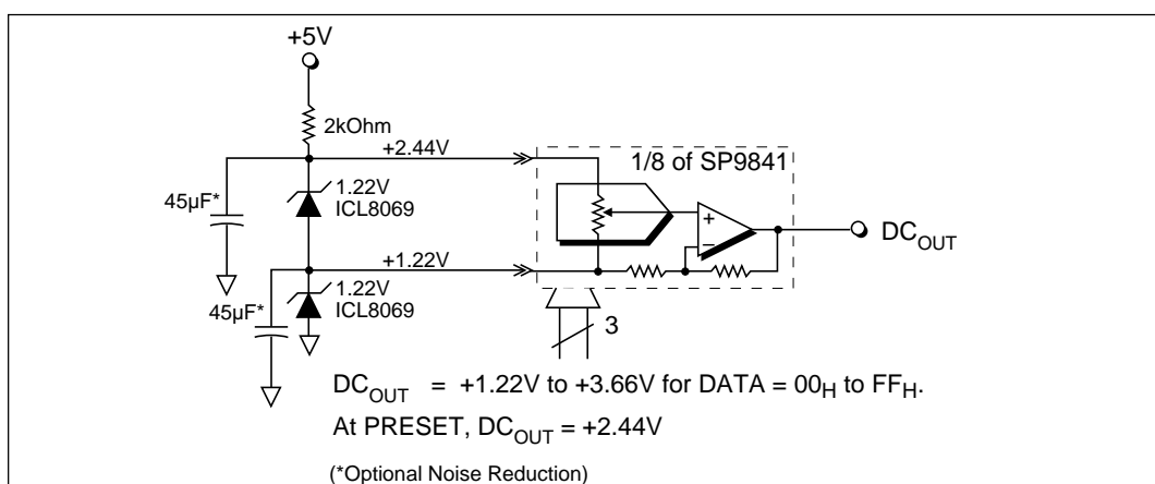
Figure 6. Pseudo Bipolar Source Generates Voltages Above and Below 2.44V.
