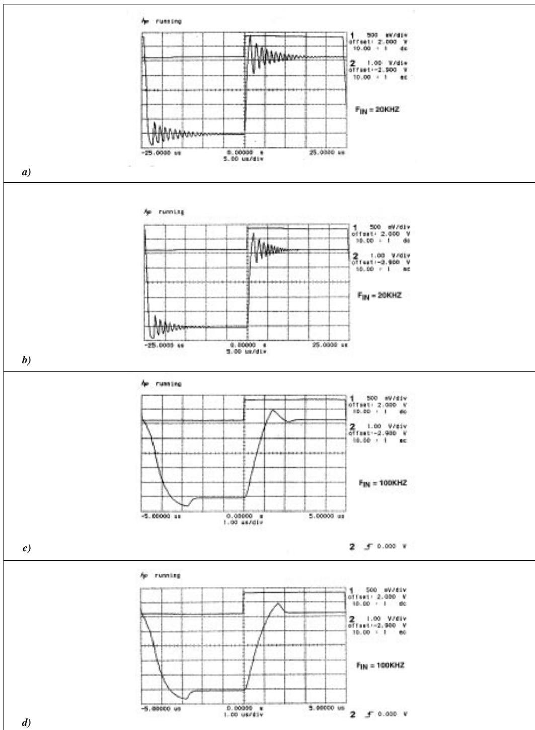
Plot 22. Pulse Response — a) C_{LOAD} = 4,700\text{pF} ; b) C_{LOAD} = 4,700\text{pF} , R_{LOAD} = 1\text{k}\Omega ; c) 30\ \Omega in series with C_{LOAD} = 4,700\text{pF} ; d) R_{LOAD} = 1\text{k}\Omega , 30\Omega in series with C_{LOAD} = 4,700\text{pF} .
