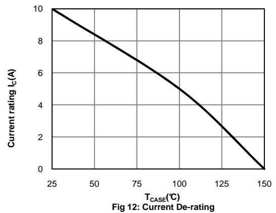
Fig 12: Current De-rating
