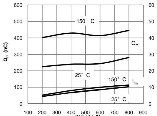
Fig 25: Diode Reverse Recovery Charge and Peak Current vs. di/dt ( V_{GE}=15V, V_{CE}=400V, I_F=5A )
