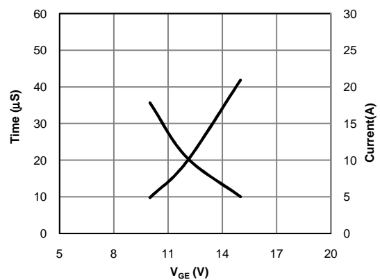
Fig 6: V_{GE} vs. Short Circuit Time ( V_{CE}=400\text{V}, T_C=25^\circ\text{C} )
