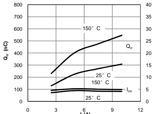
Fig 23: Diode Reverse Recovery Charge and Peak Current vs. Conduction Current ( V_{GE}=15V, V_{CE}=400V, di/dt=200A/\mu s )
