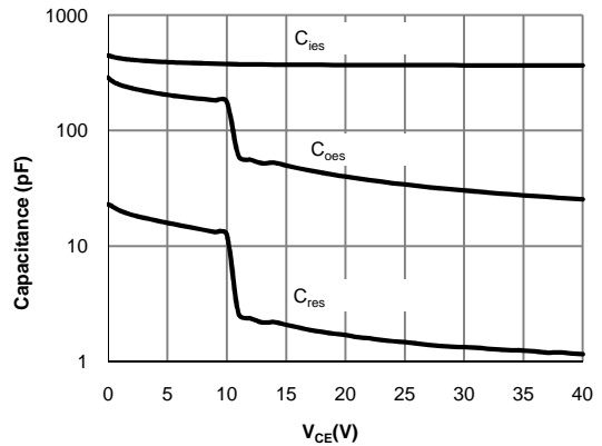
Fig 8: Capacitance Characteristic
