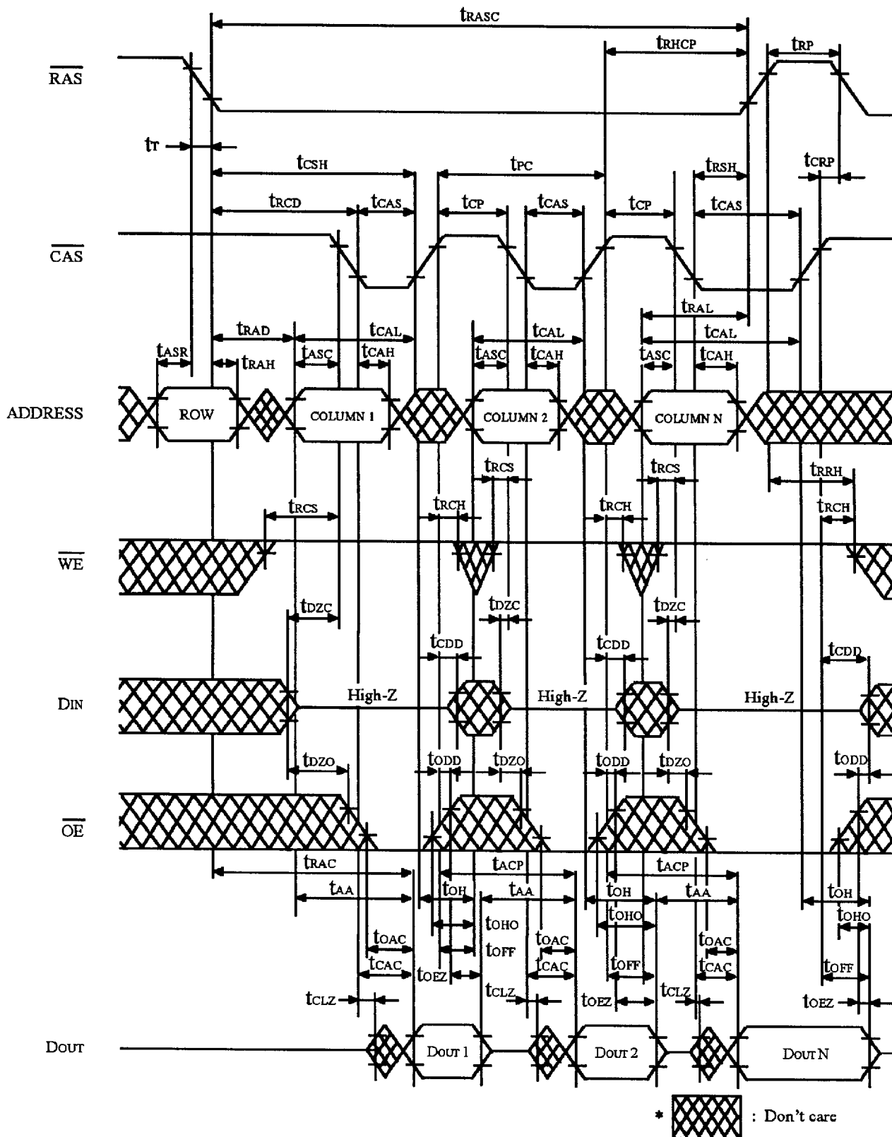
FIGURE 6. FAST PAGE MODE READ CYCLE
