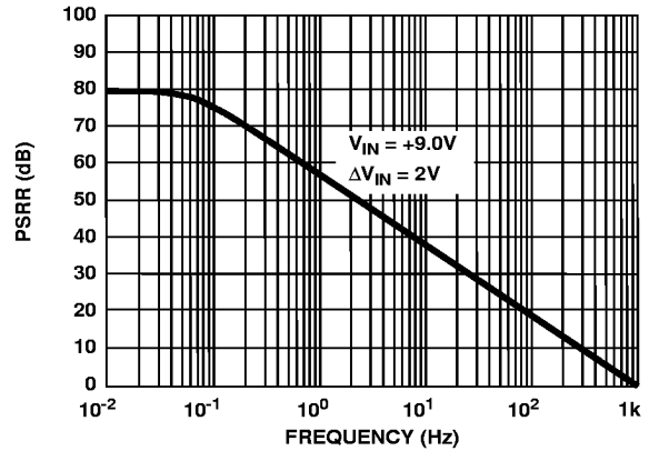
FIGURE 4. INPUT POWER SUPPLY REJECTION RATIO
