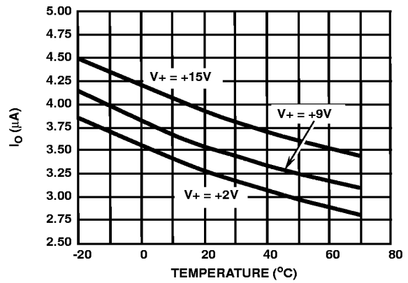
FIGURE 6. QUIESCENT CURRENT AS A FUNCTION OF TEMPERATURE
