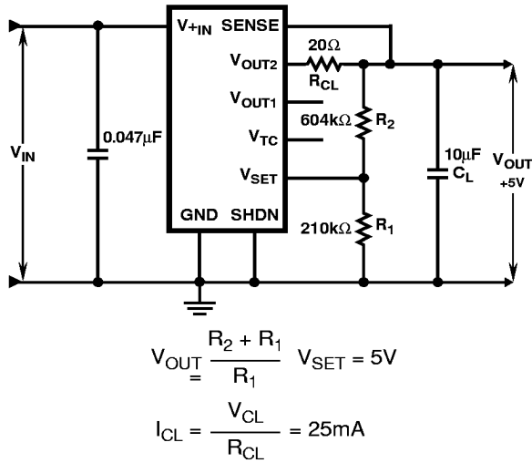
FIGURE 8. POSITIVE REGULATOR WITH CURRENT LIMIT
