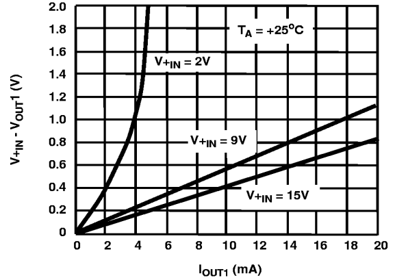
FIGURE 2. V_{OUT1} INPUT-OUTPUT DIFFERENTIAL vs OUTPUT CURRENT
