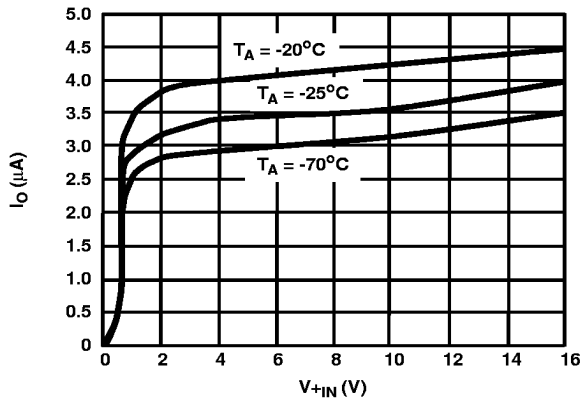
FIGURE 5. QUIESCENT CURRENT AS A FUNCTION OF INPUT VOLTAGE
