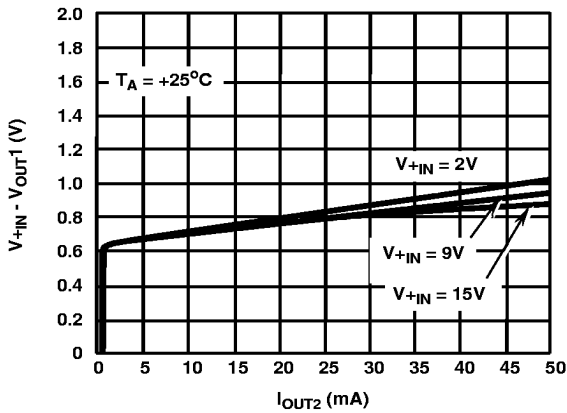
FIGURE 3. V_{OUT2} INPUT-OUTPUT DIFFERENTIAL vs OUTPUT CURRENT
