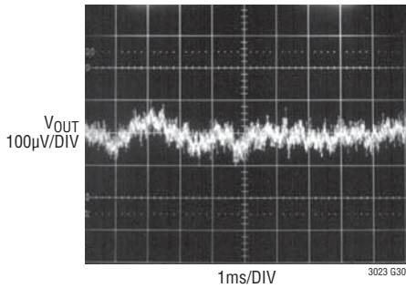
10Hz to 100kHz Output Noise C_{BYP} = 1000pF
