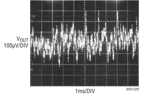
10Hz to 100kHz Output Noise C_{BYP} = 100pF
