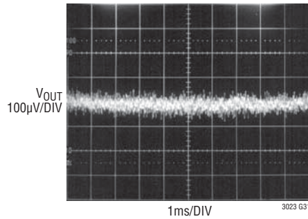
10Hz to 100kHz Output Noise C_{BYP} = 0.01\mu F
