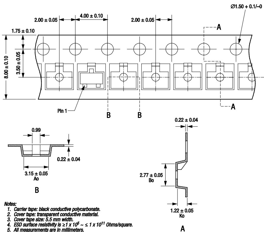
Figure 16. SOT-23 Tape and Reel Dimensions
