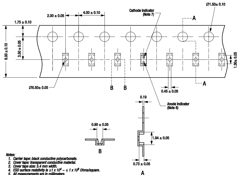
Figure 10. SC-79 Tape and Reel Dimensions
