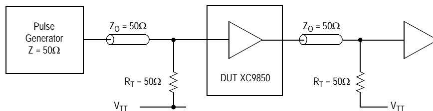
Figure 5. XC9850 AC Test Reference (LVCMOS Outputs)
