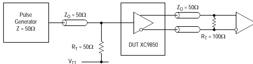
Figure 4. XC9850 AC Test Reference (LVDS Outputs)
