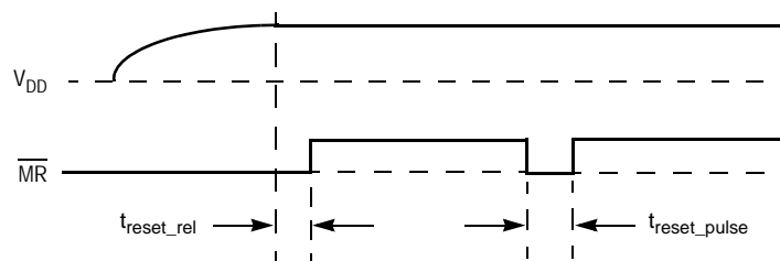
Figure 2. MR Operation
