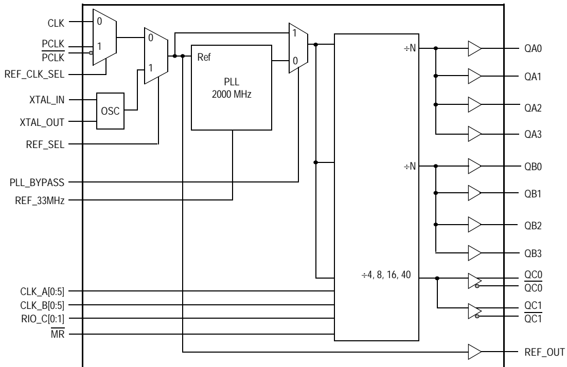
Figure 1. XC9850 Logic Diagram
