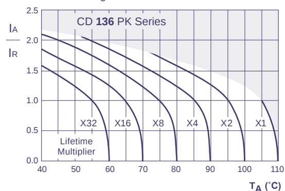
Lifetime Diagram
