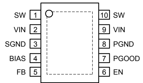
10-Pin ePad MSOP (MM)
