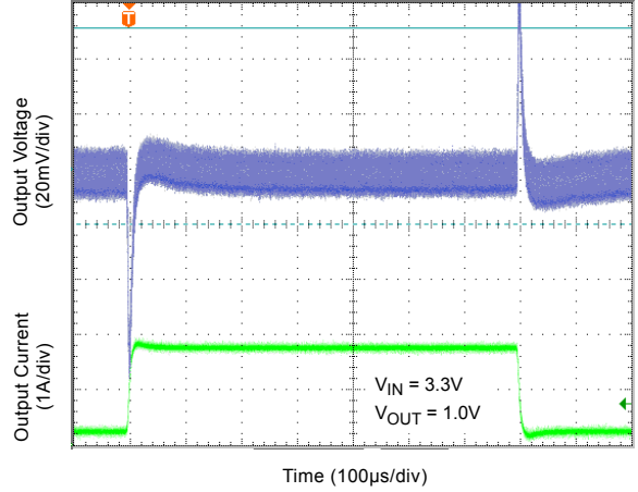
Load Transient
