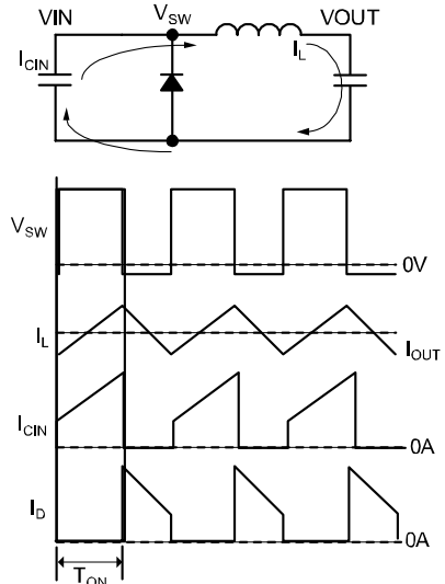
Figure 3. On-Time
